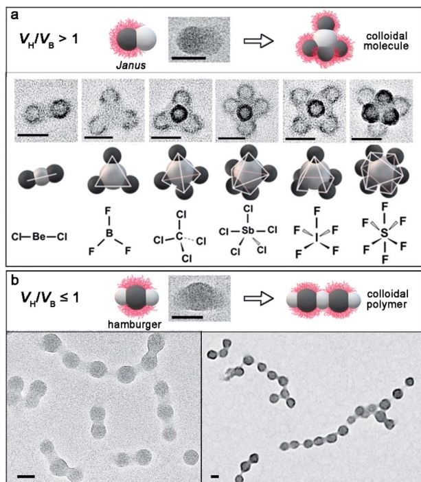
Fig. 3 (a) Self-assembly of the \text{PDMA}_{70}\text{-}b\text{-PBzMA}_{96}\text{-}b\text{-PHPMA}_{319} triblock terpolymer toward CMs with V_H/V_B > 1 ; inset shows the cryo-TEM image of the unstable Janus intermediate. TEM images of varied \text{PDMA}\text{-}b\text{-PBzMA}\text{-}b\text{-PHPMA} CMs after PTA-staining; inset shows schematic structures and molecules. (b) Illustrative self-assembly of \text{PDMA}\text{-}b\text{-PBzMA}\text{-}b\text{-PHPMA} at V_H/V_B \leq 1 . Cryo-TEM (bottom, left) and TEM images (bottom, right) after PTA-staining of \text{PDMA}_{70}\text{-}b\text{-PBzMA}_{321}\text{-}b\text{-PHPMA}_{169} colloidal chains via the “Hamburger” (insert) structure. Scale bars are 50 nm.
