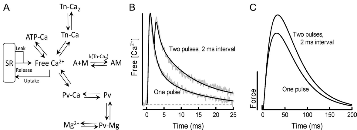
Figure 1. Simulation of the effects of doublet stimulation on cytosolic free Ca 2+ and force production. (A) Graphical depiction of the model of Ca 2+ distribution and force generation. The model incorporates both a constant Ca 2+ leak and stimulus-induced, transient Ca 2+ release from the SR. In the myoplasm, Ca 2+ is distributed among (i) TnC (Tn), with two, sequentially filled Ca 2+ binding sites, forming Tn-Ca when one Ca 2+ is bound and Tn-Ca 2 when both sites are occupied; (ii) parvalbumin (Pv), which has two equivalent Ca 2+ -binding sites per molecule that also bind Mg 2+ ; (iii) ATP; and (iv) unbound or free Ca 2+ . Ca 2+ is removed from the myoplasm via the SR Ca 2+ pump. Force generation involves the binding of myosin cross-bridges (M) to binding sites on actin (A) to form the force-generating actomyosin complex (AM). AM formation was regulated by Tn-Ca 2 , which was achieved by setting the concentration of available actin sites equal to [Tn-Ca 2 ]. (B) Comparison of recorded Ca 2+ transients (gray uneven lines) and modeled free Ca transients (black smooth lines). Two records are shown, the response to a single stimulus pulse and the response to two stimulus pulses separated by 2 ms. The experimental records are the mean of records from four fibers with amplitude scaled by the maximum amplitude in response to the first stimulus pulse. (C) Simulated force responses to one pulse and to two pulses separated by 2 ms.
