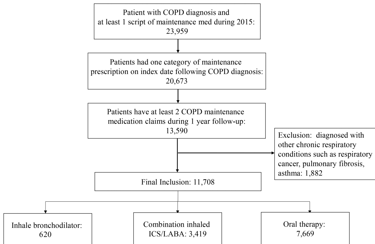
Figure 1 Patient flowchart.
