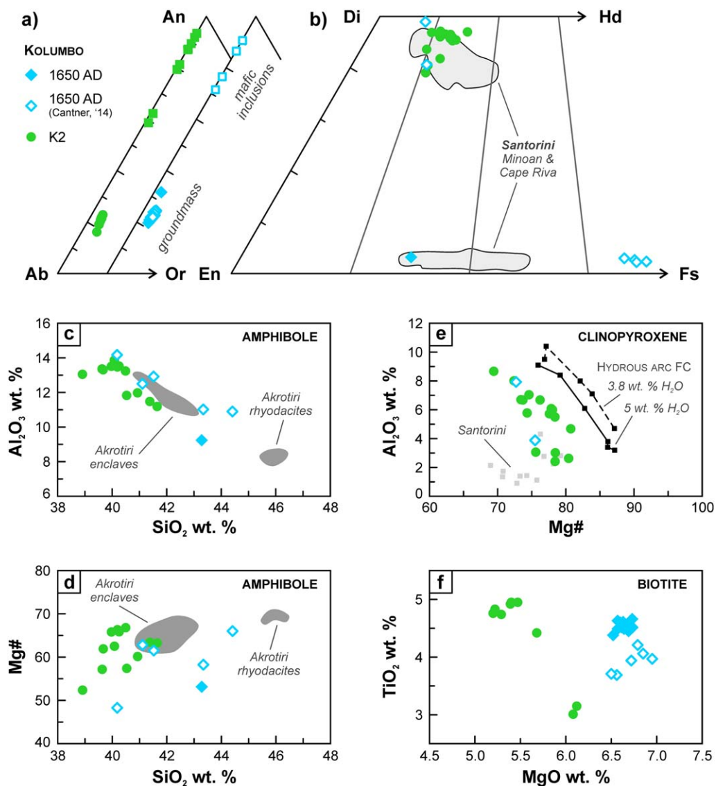
Figure 4. Compositions of (a) plagioclase, (b, e) pyroxene, (c, d) amphibole, and (f) biotite in K2 and 1650 AD pumice samples compared with Santorini Minoan and Cape Riva mineral data (light grey squares and fields [Huijsmans, 1985; Cottrell et al. , 1999; Druitt et al. , 1999]). Data for the 1650 AD pumices are from Cantner et al. [2014] and are shown as open symbols. Also included in Figures 4c and 4d is the range of amphibole compositions in the Akrotiri rhyodacites and enclaves on Santorini [Mortazavi and Sparks, 2004]. The composition of clinopyroxene formed during hydrous crystallization experiments of primitive arc magmas is shown for reference in Figure 4e [Müntener et al. , 2001].
