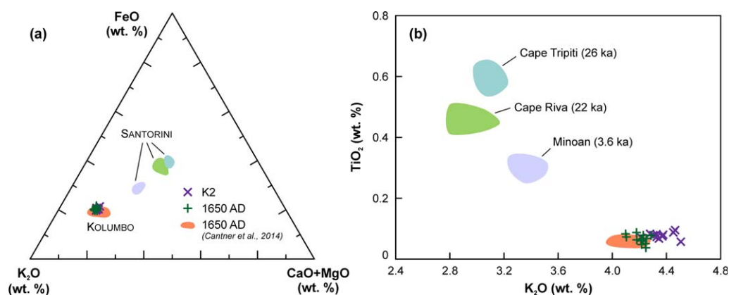
Figure 3. Glass compositions for the K2 and 1650 AD pumice samples: (a) FeO – K 2 O – CaO + MgO ternary diagram; (b) TiO 2 versus K 2 O diagram. Data for the 1650 AD pumice from Cantner et al. [2014] are included (orange field). Glass compositions of eruptive products from the three most recent major Plinian eruptions from Santorini (Cape Tripiti, Cape Riva, Minoan) are shown for reference; data are from Vinci [1985], Wulf et al. [2002], Aksu et al. [2008] and Fabbro et al. [2013]. All analyses are recalculated on a volatile-free basis normalized to 100%.
