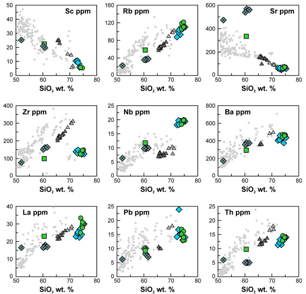
Figure 6. Variation diagrams of selected trace elements versus SiO 2 for the Kolumbo sample suite in comparison with the range of Santorini volcanic products. For Santorini, the recent Kameni dacites (dark grey triangles) and Minoan Tuff (light grey triangles) are highlighted. Symbols and data sources as in Figure 5.
