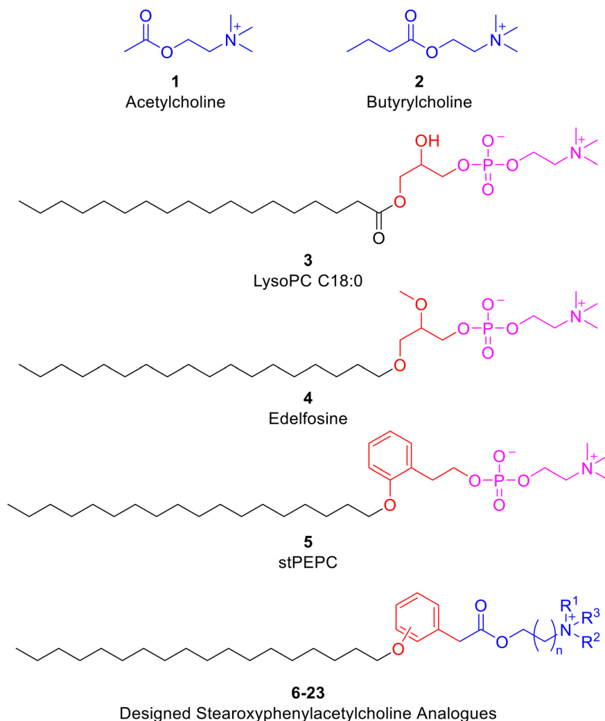
Fig. 3 Previously known bioactive compounds and the design rational of the targeted derivatives of phenylacetylcholine analogues.
