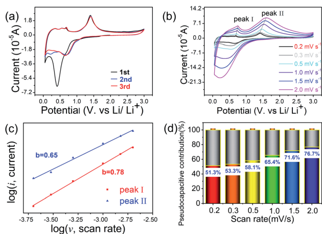
Fig. 6 Electric properties of ZnS@NC-H. (a) Cyclic voltammogram curves of initial three cycles at a scan rate of 0.2 \text{ mV s}^{-1} between 0.05 and 3.0 V vs. Li/Li + . (b) CV curves at different scan rates of 0.2, 0.3, 0.5, 1.0, 1.5, 2.0 \text{mV s}^{-1} . (c) b -Value analysis based on the relationship between the peak currents and the scan rates. (d) Normalized contribution ratios of pseudocapacitance (in color) and diffusion-controlled (in gray) capacities at different scan rates.
