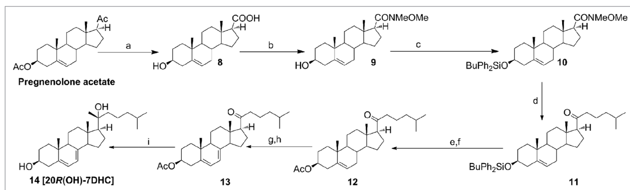
Figure 3. The synthesis of 20R(OH)7DHC.
