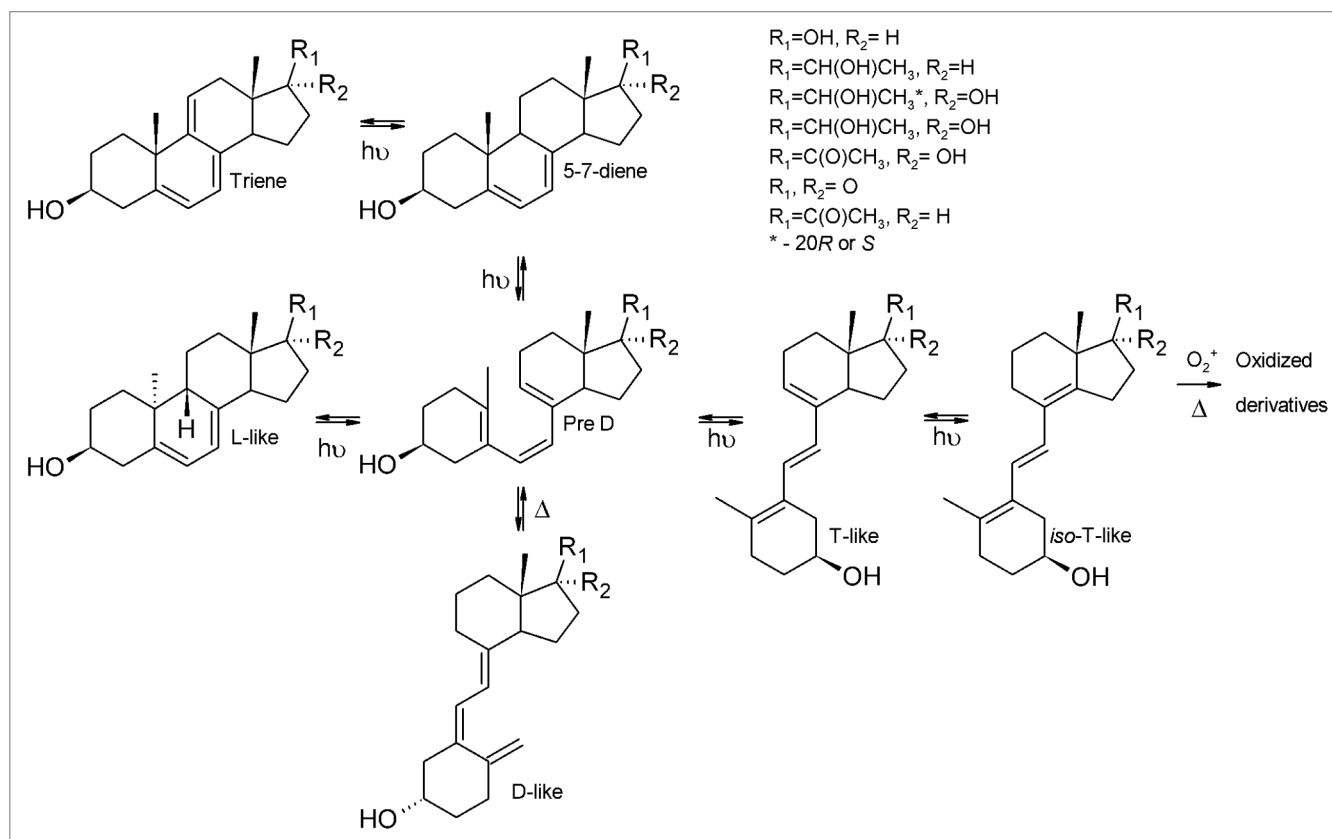
Figure 5. UVB-induced transformation of steroidal 5,7-dienes to secosteroids.
