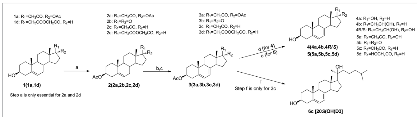
Figure 2. The synthesis of the 5,7-diene precursors of secosteroid analogs.
