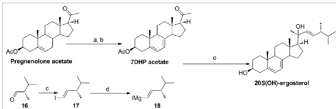
Figure 4. The plausible synthetic route of 20(OH)ergosterol.
