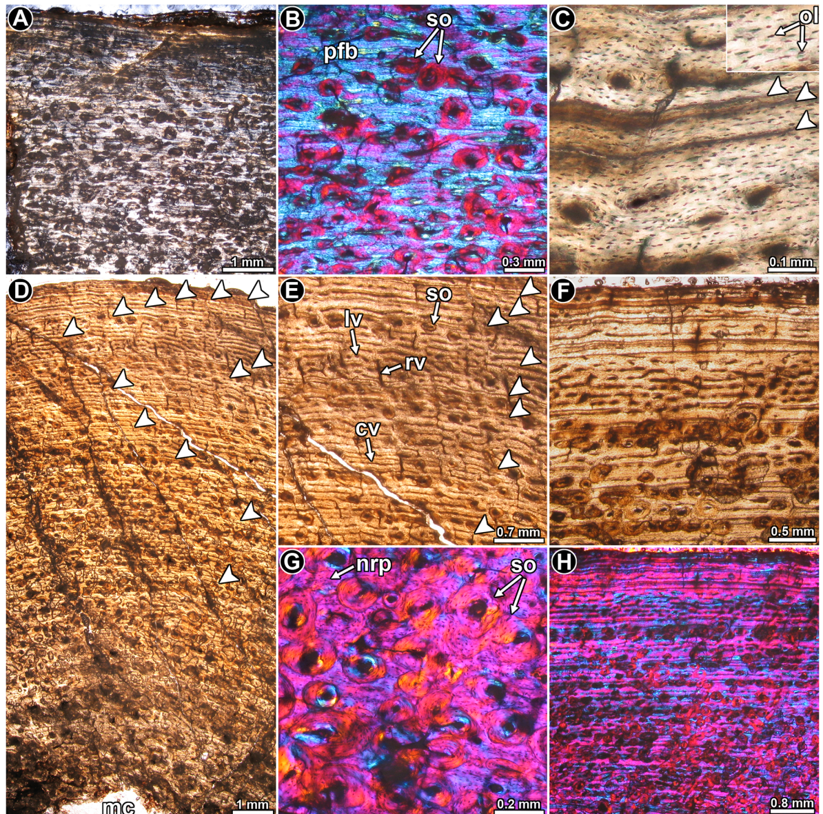
Fig 7. Femur histology of Lyesaurus marayensis PVSJ 1079. (A, B) General view (A) and detail (B) of the cortical bone. Note the mass birefringence of the primary bone tissue. Polarized light (A) and polarized light with lambda compensator (B). (C) Detailed view of the primary bone tissue showing flattened osteocyte lacunae. Double and single LAGs are also observed. Normal transmitted light. (D, E) General view (D) and detail (E) of the cortex showing the arrangement of vascular canals and the relative distribution of LAGs. Normal transmitted light. (F) Enlarged view of the outer cortex. Note that the spacing between successive LAGs is reduced toward the periosteal surface. Normal transmitted light. (G) Highly remodeled portion of the cortex showing different generations of secondary osteons. Despite the relative abundance of the secondary osteons, interstitial primary bone is preserved. Polarized light with lambda compensator. (H) General view of the compact bone showing abundant secondary osteons, which are arranged in concentric rows in some areas. Polarized light with lambda compensator. Abbreviations: cv: circumferentially oriented vascular canal; nrp: non remodeled primary bone tissue; lv: longitudinally oriented vascular canal; mc: medullary cavity; ol: osteocyte lacunae; pfb: parallel fibered bone; rv: radially oriented vascular canal; so: secondary osteons.
