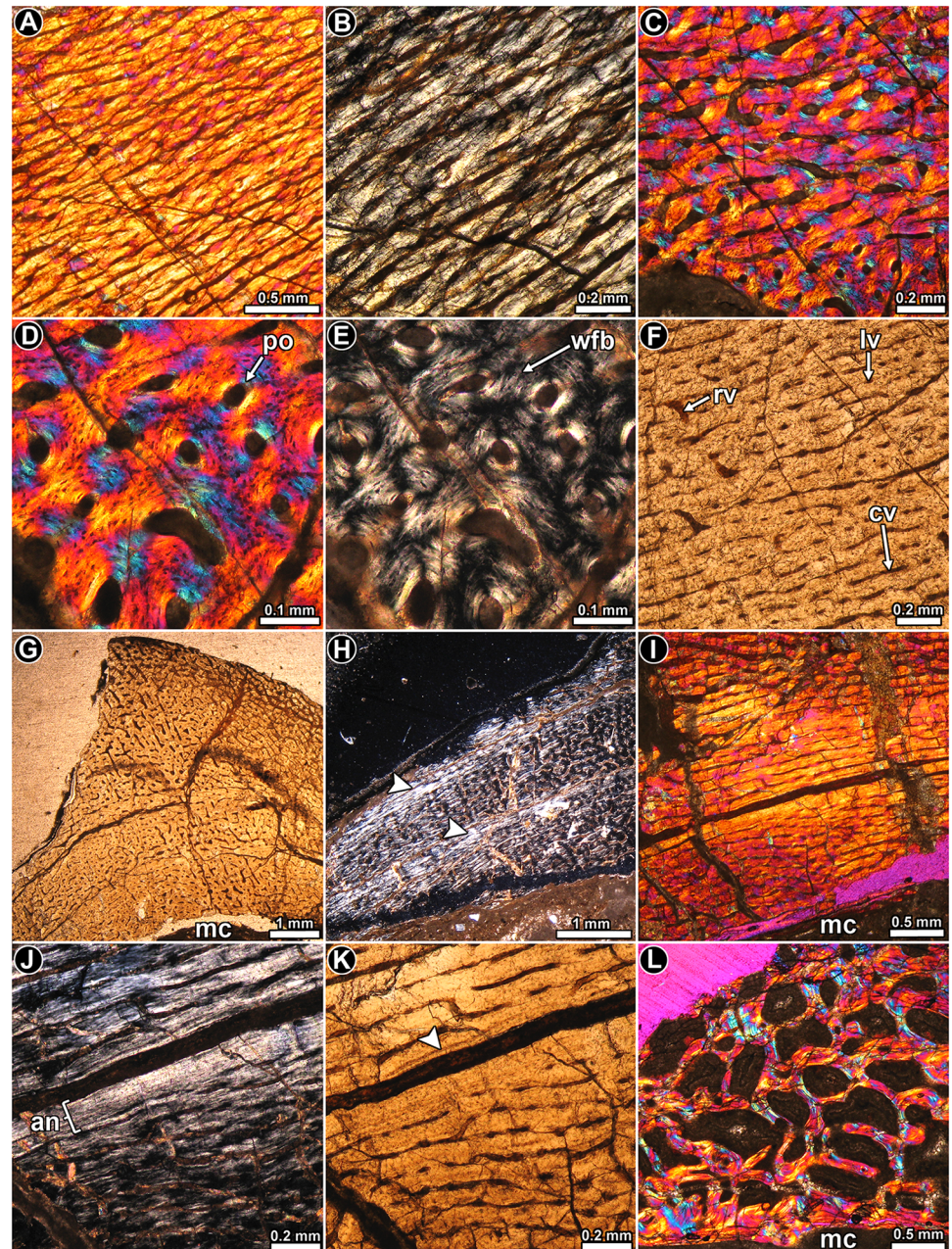
Fig 10. Femur histology of Leonerasaurus taquetrensis MPEF 1663. (A, B) General view (A) and detail (B) of the primary bone tissue, which is mostly composed of parallel fibered bone. Polarized light with lambda compensator (A) and polarized light (B). (C–E) General view (C) and detail (D, E) of coarse woven fibered bone tissue. Polarized (E) and polarized light with lambda compensator (C, D). (F) Primary bone tissue in which longitudinally oriented vascular canals predominate. Normal transmitted light. (G) General view of the compact bone showing relative abundance of radial vascular canals. Normal transmitted light. (H) General view of the cortex in which two poorly defined annuli occur (arrowheads). Note that each annulus exhibits a higher degree of birefringence. Polarized light. (I–K) General view (I) and detail (J, K) of a single annulus formed in the inner cortex. Note the presence of a single LAG (arrowhead). The broken surface corresponds to a second LAG. Polarized light with lambda compensator (I), polarized light (J) and normal light (K). (L) Cancellous bone in the perimedullary region. Bony trabeculae are composed of lamellar bone deposited during different episodes of secondary remodeling. Polarized light with lambda compensator. Abbreviations: an: annulus; cv: circumferentially oriented vascular canal; lv: longitudinally oriented vascular canal; mc: medullary cavity; po: primary osteon; rv: radially oriented vascular canal; wfb: woven fibered bone.
