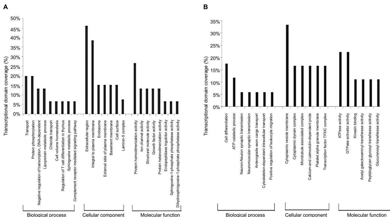
Figure 1 GO analysis of differentially expressed genes with dose-dependent relationships Notes: (A) GO analysis of upregulated genes with dose-dependent relationships. (B) GO analysis of downregulated genes with dose-dependent relationships. Abbreviations: GO, Gene Ontology.
