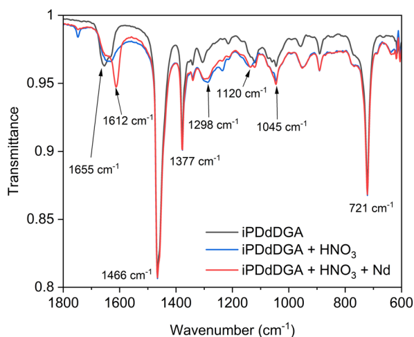
Fig. 8 FTIR spectra obtained for the iPDdDGA organic phase ( 0.1 \text{ mol L}^{-1} DGA in n -dodecane + 5 vol% 1-octanol) before extraction, after contact with 3 \text{ mol L}^{-1} \text{ HNO}_3 , and after contact with 10 \text{ mmol L}^{-1} \text{ Nd(NO}_3)_3 dissolved in 3 \text{ mol L}^{-1} \text{ HNO}_3 . [\text{H}^+]_{\text{org}} = 0.36 \text{ mol L}^{-1} , [\text{Nd}^{3+}]_{\text{org}} = 10 \text{ mmol L}^{-1} .
