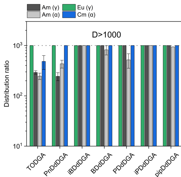
Fig. 4 Distribution ratios for extraction of Eu, Am, and Cm with diglycolamides. Aqueous phase: 18 mmol L -1 Ln(III) + 50 kBq mL -1 of 152 Eu, 241 Am, and 244 Cm each dissolved in HNO 3 solution with initial concentration 3 mol L -1 . Organic phase: 0.1 mol L -1 diglycolamide extractant dissolved in n -dodecane + 5 vol% 1-octanol. Shaking time: 15 min. Temperature: 20 °C.
