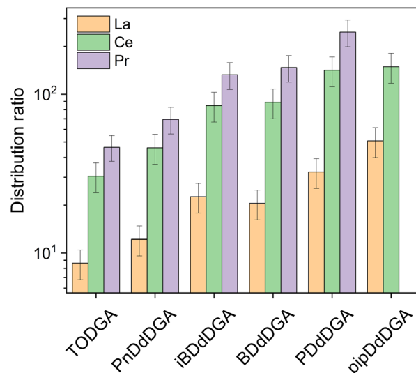
Fig. 5 Distribution ratios for extraction of lanthanides with diglycolamides. Aqueous phase: 18 mmol L -1 Ln(III) + 50 kBq mL -1 of 152 Eu, 241 Am, and 244 Cm each dissolved in HNO 3 solution with initial concentration 3 mol L -1 . Organic phase: 0.1 mol L -1 diglycolamide extractant dissolved in n -dodecane + 5 vol% 1-octanol. Shaking time: 15 min. Temperature: 20 °C.
