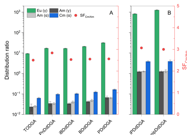
Fig. 6 Distribution ratios for stripping of Eu, Am, and Cm with SO 3 -Ph-BTBP. Organic phase: 0.1 mol L -1 diglycolamide extractant dissolved in n -dodecane + 5 vol% 1-octanol, loaded from a solution containing 18 mmol L -1 Ln(III) (A) or 10 -5 mol L -1 Eu(III) (B) + 50 kBq mL -1 of 152 Eu, 241 Am, and 244 Cm each dissolved in 3 mol L -1 HNO 3 solution. Aqueous phase: 10 mmol L -1 SO 3 -Ph-BTBP dissolved in 0.3 mol L -1 HNO 3 solution. Shaking time: 30 min. Temperature: 20 °C.
