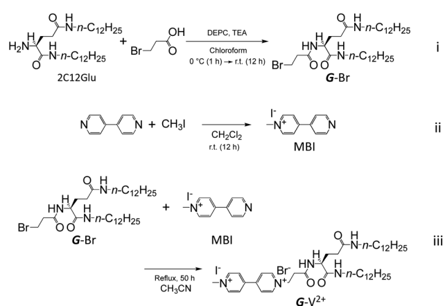
Scheme 1 Synthesis of L-glutamic acid derivatives, G\text{-V}^{2+} .
