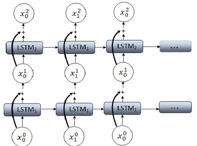
Fig. 2. The architecture of Stacked LSTM.
