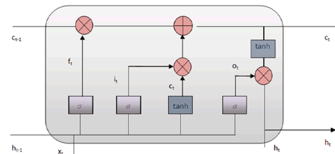
Fig. 1. The architecture of LSTM.
