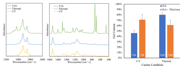
Fig. 4 FTIR traces for crosslinked Ter3 ( F_{\text{C13MA}} = 0.75 , F_{\text{FMA}} = 0.17 , F_{\text{EGDEMA}} = 0.08 ) samples with single crosslinking using BM : FMA (Diels–Alder – DA) loading of 0.1 and gel content chart for UV and thermally cured samples.
