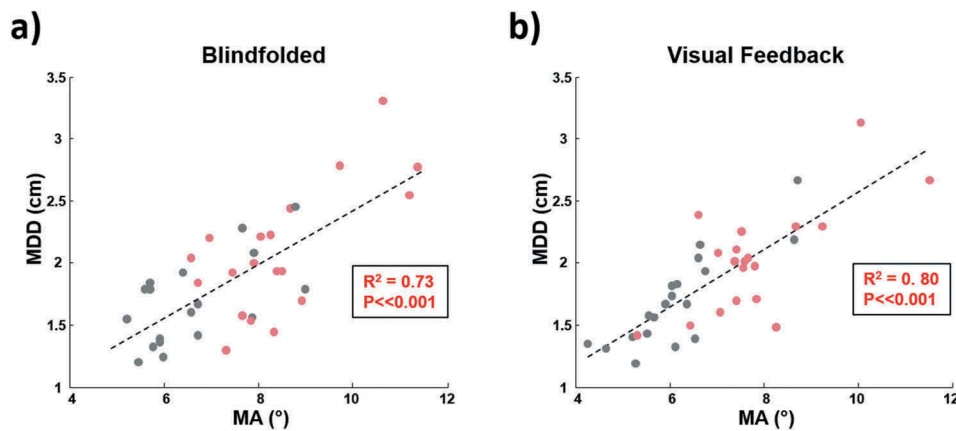
Figure 5. Scatter plots of MDD in the two conditions (Blindfolded and visual feedback; panels a and b respectively). Correlation between the variables is statistically significant in both conditions and the R2 values are indicated.
