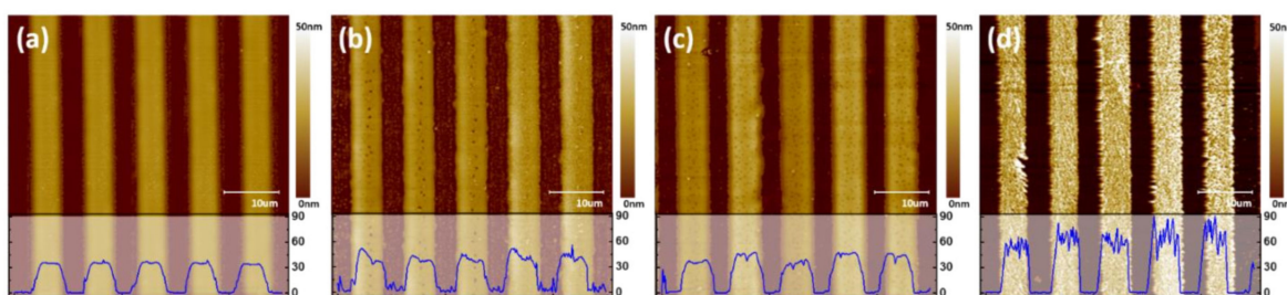
Figure 7. AFM images of sublimation transferred patterns after the drying process (a) at room temperature, (b) 30 °C, (c) 50 °C, and (d) 80 °C in a vacuum chamber. Insets are cross-sectional data, respectively.
