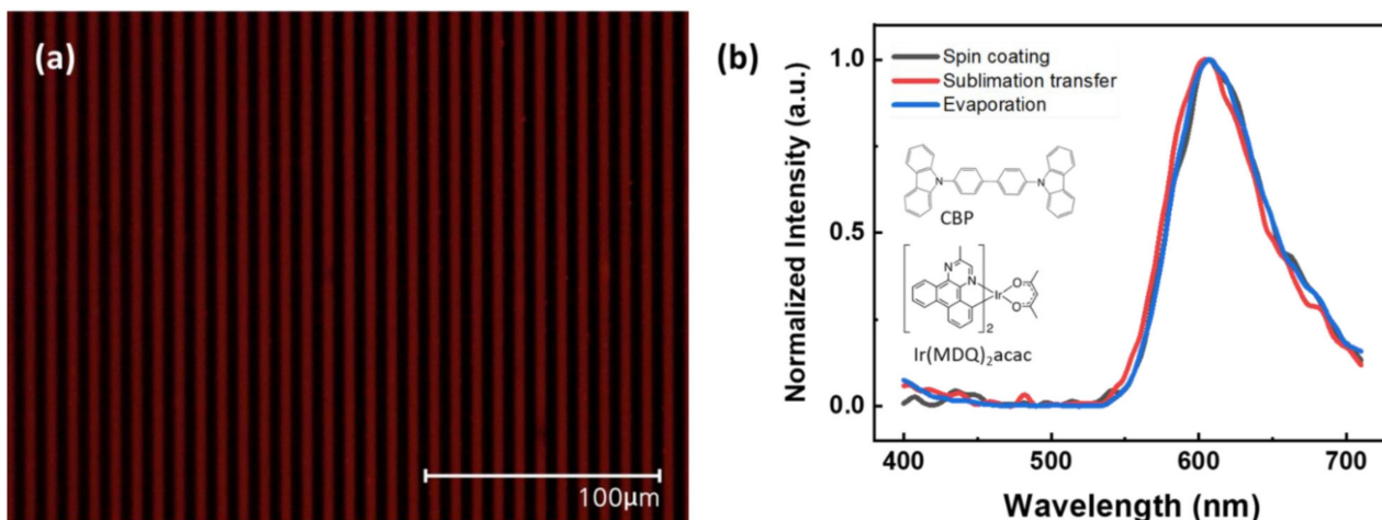
Figure 8. (a) OM image with UV exposure of sublimation transferred pattern. (b) Normalized PL spectra at an excitation wavelength of 365 nm, according to the patterning methods; sublimation transfer, evaporation, and spin-coating. Insets are the chemical structure of the emitting materials; CBP and Ir(MDQ) 2 acac.
