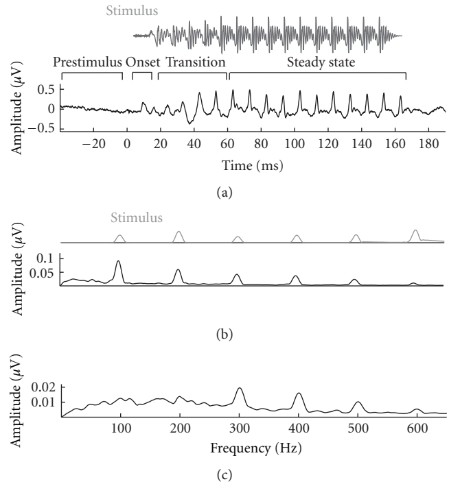
FIGURE 1: The stimulus /da/ (gray) is displayed with its response (black) in time and frequency domains. (a) Time domain. The response represents an average of 17 older adults (ages 60 to 67) all of whom have audiometrically normal hearing. The periodicity of the stimulus is reflected in the response with peaks repeating every ~10 ms (the F_0 of the vowel /a/). (b) and (c) Frequency domain. Fast Fourier transforms were calculated over the steady-state region of the response, showing frequency energy at the F_0 (100 Hz) and its integer harmonics for responses obtained by adding (b) and subtracting (c) responses to alternating polarities.
