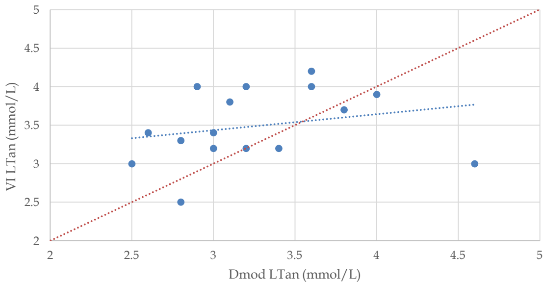
Figure 4. Visualization of Bland & Altman’s “line of agreement” (orange line) using mock data. This is analogous to a line of y=x when two LTan prediction methods are plotted against one another. Both Bland-Altman analysis and Lin’s Concordance Correlation Coefficient are means of quantifying the degree of scatter (blue points) about the line of agreement between two measures of the same quantity. The two methods plotted here are linearly correlated (blue line) despite demonstrating poor agreement.
