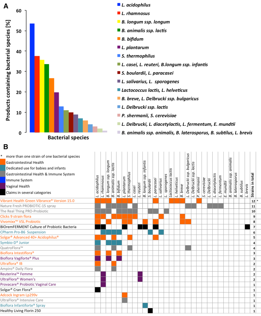
Fig. 2 Bacterial distribution in probiotics. a Constituting organisms. Bacterial species contained in probiotics belonged to the genera Lactobacillus with 15 species, Bifidobacterium with 8 species, Streptococcus thermophilus , Enterococcus mundtii and Propionibacterium shermanii . The yeast Saccharomyces was represented with two species. b Health claims and association with bacterial composition. Each product was grouped into one health category as described above and bacterial strains were listed. For the complete figure see Additional file 1: Figure S1.1 and Additional file 2: Figure S1.2
