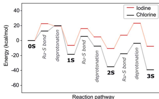
Fig. 4 Energy evolution of the trithiolato complex 1 formation in presence of chlorine and iodine. The transition-state barriers are presented numerically in Table S2 (ESI†) and the NEB pathways can be found in Fig. S6 (ESI†).
