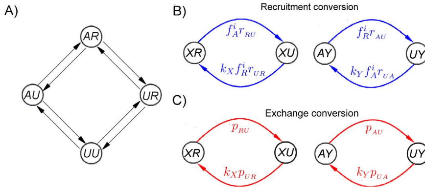
Figure 3. Transitions for the reduced 4-state model. (A) Transitions among the 4 distinct nucleosome states (i.e., AR , UR , AU , and UU ) in the 4-state model. The time step is small enough that at most only one modification site of a nucleosome may change on each time step. (B) Transition probabilities between nucleosome states via recruitment conversions, where X can either be A or U while Y can either be R or U . k_X ( k_Y ) = 2 if X ( Y ) is U , otherwise k_X ( k_Y ) = 1. Thus, as an example, the transition probability from the AR state to the AU state is the same as that from the UR state to the UU state. (C) Transition probabilities between nucleosome states via exchange conversions, where X can either be A or U while Y can either be R or U .
