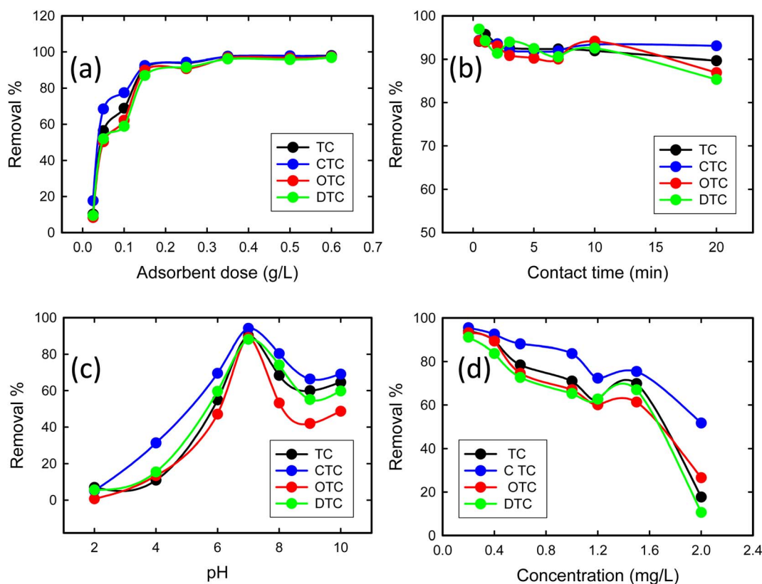
Fig. 5 (a) Effect of the adsorbent dose on the adsorption of tetracyclines from aqueous solutions onto the GO/Co-Fe composite ( C_0 = 200 ppb, t = 30 min, shaking = 250 rpm, T = 25 °C). (b) Effect of time on the adsorption of tetracyclines from the aqueous solution by GO/Fe-Co ( C_0 = 200 ppb, GO/Co-Fe = 0.15 \text{ g L}^{-1} , shaking = 250 rpm, T = 25 °C, pH = 7). (c) Effect of pH on the adsorption of tetracyclines from the aqueous solution by GO/Co-Fe ( C_0 = 200 ppb, GO/Co-Fe = 0.15 \text{ g L}^{-1} , t = 0.5 min, shaking = 250 rpm, T = 25 °C). (d) Effect of concentration on the adsorption of tetracyclines from the aqueous solution by GO/Co-Fe ( C_0 = 200 ppb, GO/Co-Fe = 0.15 \text{ g L}^{-1} , t = 0.5 min, pH = 7, shaking = 250 rpm, T = 25 °C).
