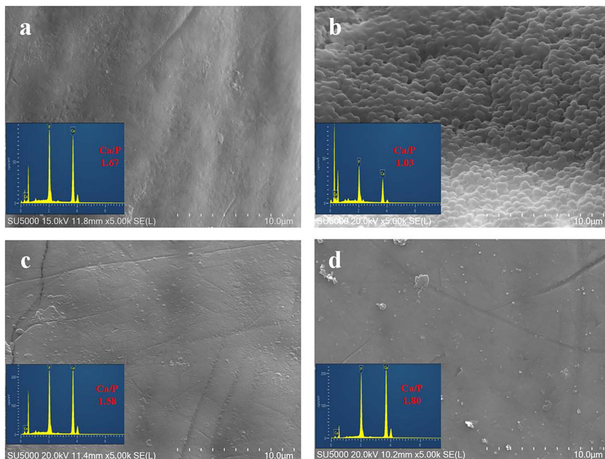
Fig. 5 SEM images and elemental analysis of (a) negative control group, (b) positive control group, (c) TiO 2 -HAP treatment group and (d) TiO 2 -HAP prevention group.
