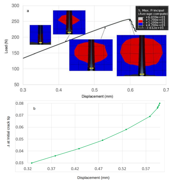
Figure 10. CZS prediction of the fracture process for D230 + 5 wt% MX-257. (a) Load vs. LLD, with the corresponding maximum principal stress (MAXPS) contours shown at various points. Yellow arrows indicate the degree of separation between the nodes at the initial crack tip. (b) Separation between crack faces at the crack tip vs. LLD.
