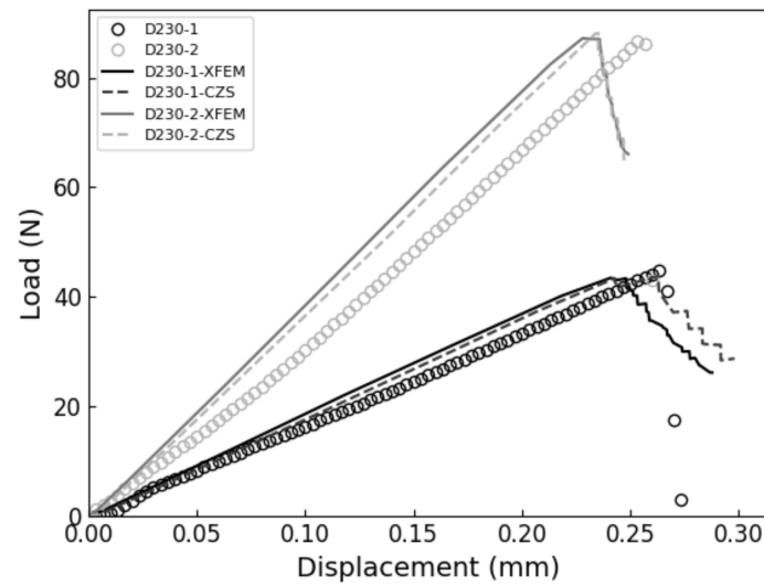
Figure 6. Experimental vs. XFEM and CZS-predicted SENB test load-displacement curves for unfilled D230 resins.
