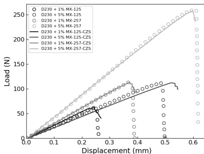
Figure 4. CZS-predicted SENB test load-displacement curves (solid lines) benchmarked against experimental data for each nanocomposite resin.
