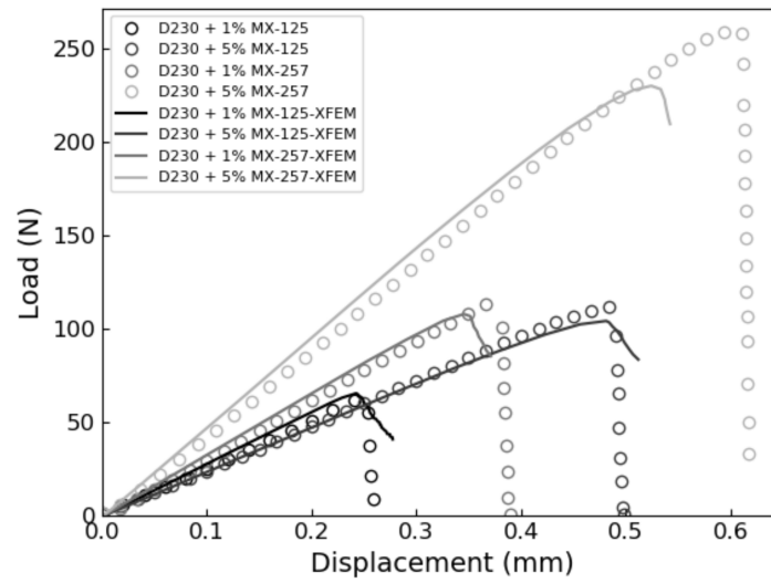
Figure 5. XFEM-predicted SENB test load-displacement curves (solid lines) benchmarked against experimental data for each nanocomposite resin.
