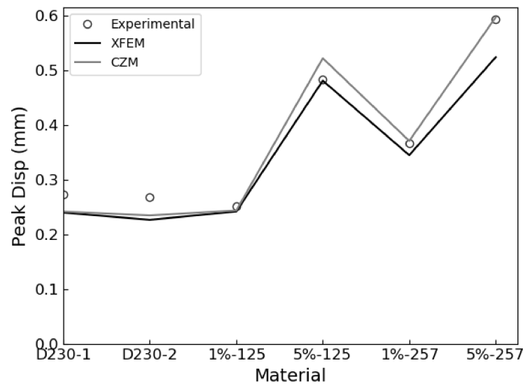
Figure 8. Experimental vs. predicted load-line displacements (LLDs) d_c for each material.
