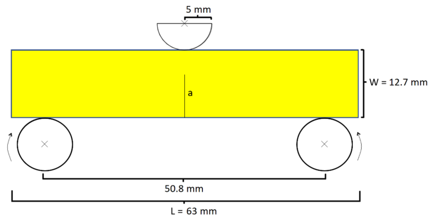
Figure 1. Configuration of the simulated SENB test apparatus within which the stationary bottom pins are rotatable.
