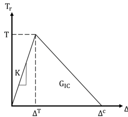
Figure 2. The linear traction–separation law (TSL) used to model damage initiation and evolution of the mode I fracture. This plot represents the c = 1 case of the truncated linear TSL.
