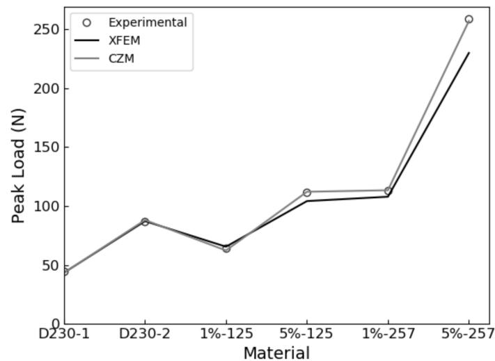
Figure 7. Experimental vs. predicted maximum loads P_{max} for each material.
