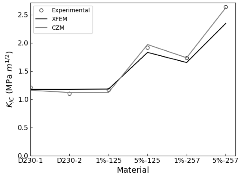
Figure 9. Experimental vs. predicted mode I fracture toughness K_{IC} for each material.
