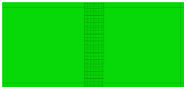
Figure 3. Close-up image of the mesh of the sub-laminate layer that was used in the CZS simulations.
