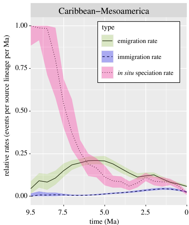
Figure 4. Within-area dispersal and speciation rates through time of Caribbean-Mesoamerica based on 100 000 biogeographic stochastic mappings under the DEC model in BioGeoBEARS. Type lines are the median values; coloured ribbons are the lower and upper quartiles (0.25 and 0.75 quantiles). (Online version in colour.)
