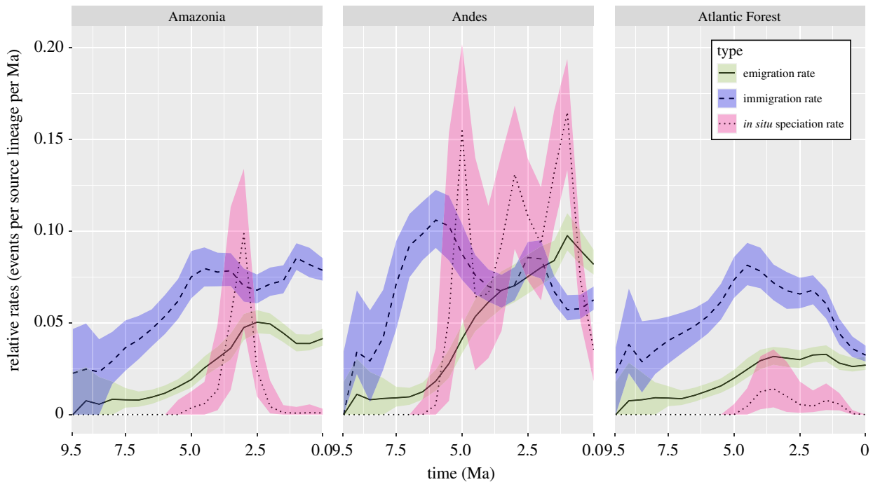
Figure 5. Within-area dispersal and speciation rates through time of Amazonia, Andes and Atlantic Forest based on 100 000 biogeographic stochastic mappings under the DEC model in BioGeoBEARS. Type lines are the median values; coloured ribbons are the lower and upper quartiles (0.25 and 0.75 quantiles). (Online version in colour.)
