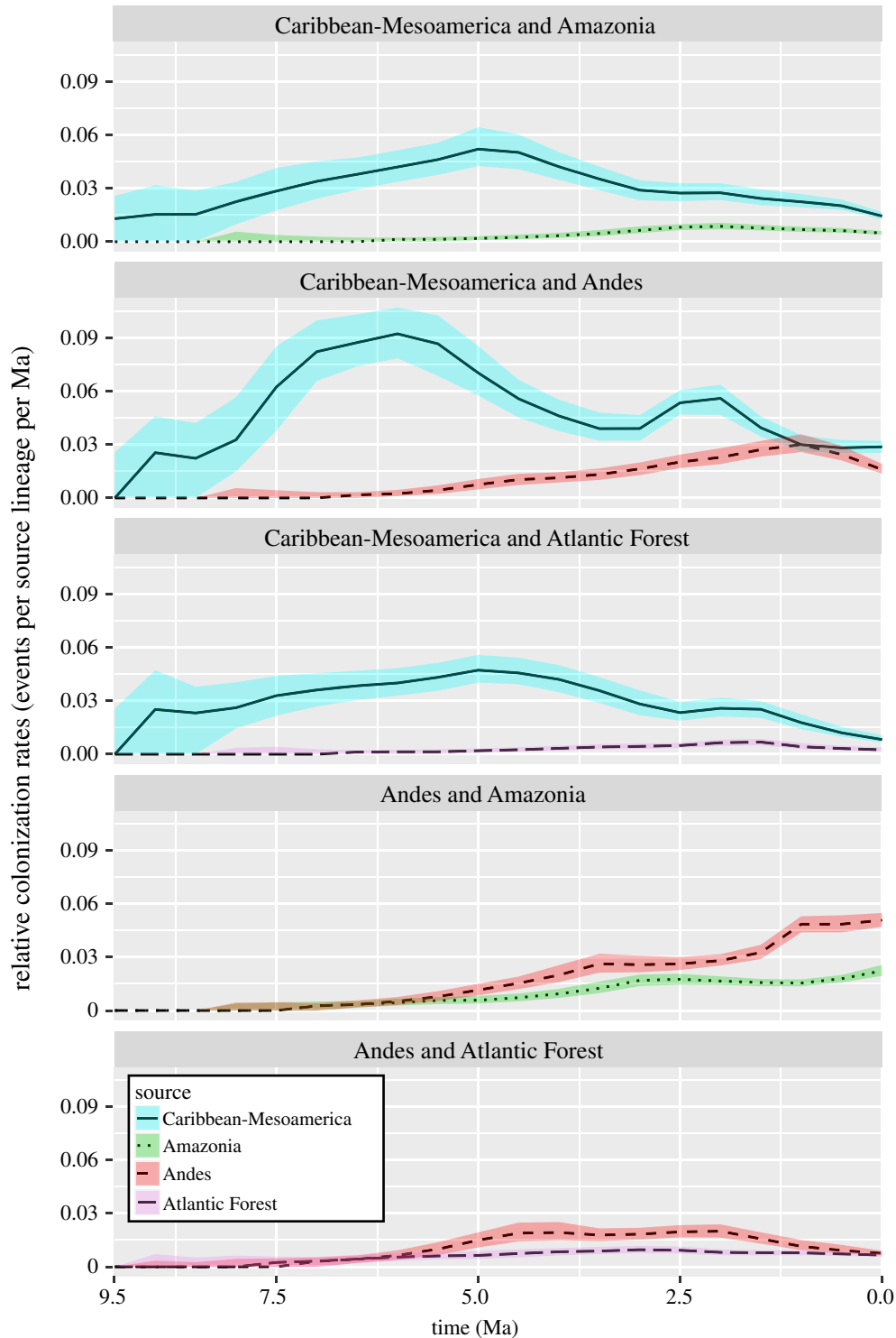
Figure 3. Dispersal rates through time based on 100 000 biogeographic stochastic mappings under the DEC model in BioGeoBEARS. Rates are displayed for selected pairs of areas. Source lines are the median values; coloured ribbons are the lower and upper quartiles (0.25 and 0.75 quantiles). (Online version in colour.)
