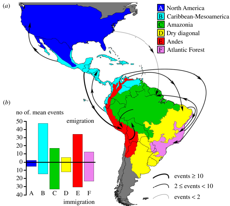
Figure 2. Summary of major Xylophanes dispersal events, average number of dispersal events between two areas based on 100 000 biogeographic stochastic mappings under the DEC model in BioGeoBEARS. (a) The highest emigration and the highest immigration of each area are summarized on the map. The width and shape of lines represent the estimated average number of dispersal events. (b) Bar chart showing average number of emigration and immigration events of each area. Complete average dispersal events between each type shown in electronic supplementary material, appendix S5. (Online version in colour.)
