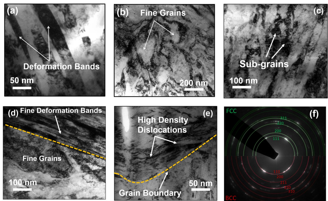
Figure 3. Transmission electron microscope (TEM) images for (a) ultra-fine grain steel; bimodal steel showing (b) finer grains of the order of 200–400 nm, (c) fine sub grains, (d) fine deformation bands, (e) high density dislocation along the grain boundary, and (f) selected electron diffraction pattern (SADP). The UFG steel showed elongated deformation bands with high density dislocation. SADP for bimodal specimen showed both FCC and BCC phases. The BCC phase corresponds to martensite.
