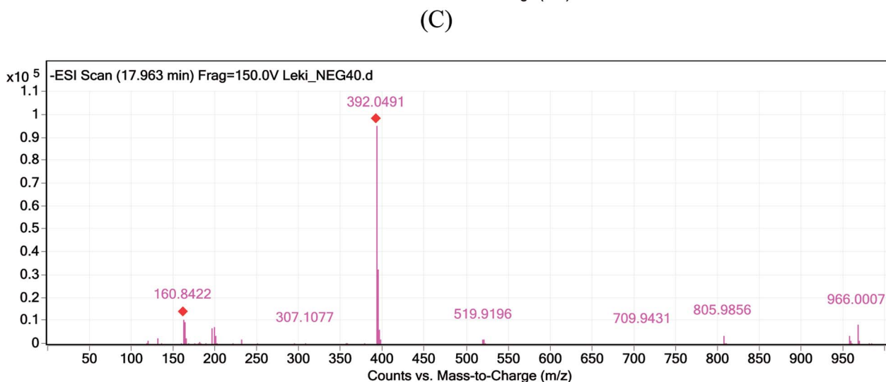
Fig. 6 Chromatogram DAD of indapamide (6) and dihydralazine (1) and their degradation product (2–5, 7) in borate buffer of pH 10 (A); negative ion ESI LC-MS of degradation product 2 of indapamide (B); negative ion ESI LC-MS of degradation product 5 of indapamide (C); CID off set 10 V.
