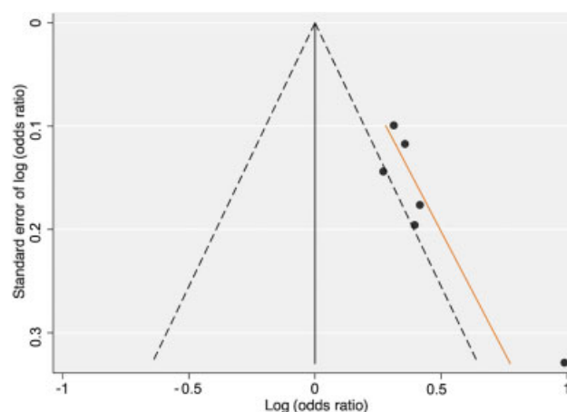
Fig. 3 Funnel plot of studies included in meta-analysis investigating the risk of ischemic stroke per 5 \mu\text{mol/L} increase in homocysteine.
