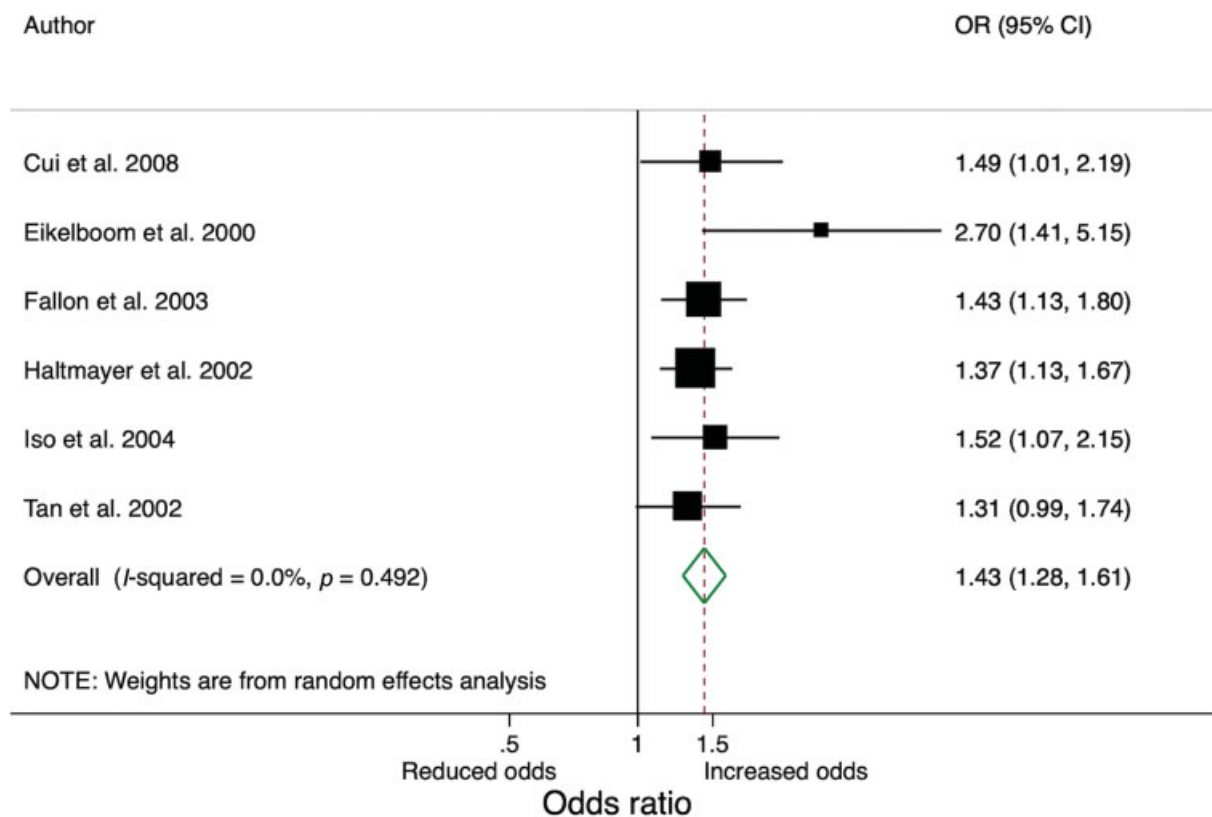
Fig. 2 Forest plot of risk of ischemic stroke per 5 \mu\text{mol/L} increase in plasma homocysteine. CI, confidence interval; OR, odds ratio.
