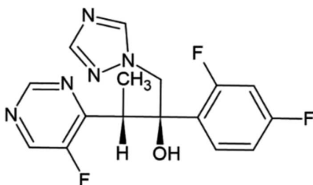
Fig. 1 Structure of voriconazole.
