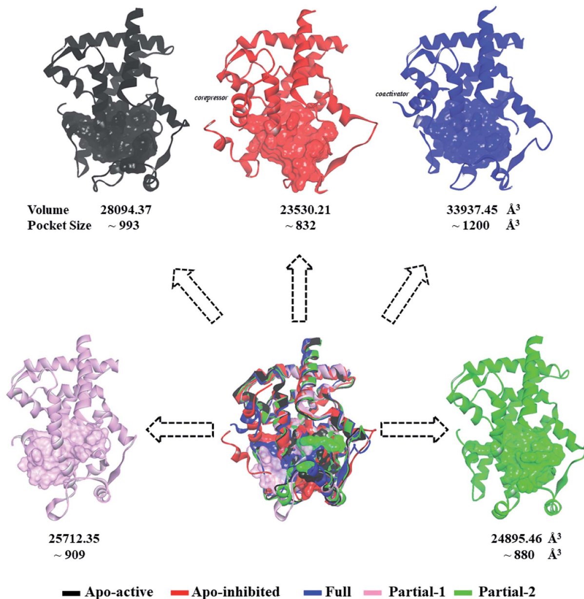
Fig. 2 Superimposition of various representative PPAR \gamma -LBD conformations which were derived from simulation trajectories by using root mean-square difference (RMSD) clustering. The volumes and pocket sizes were separately determined by Discovery Studio client 35 and Fpocket program. 50
