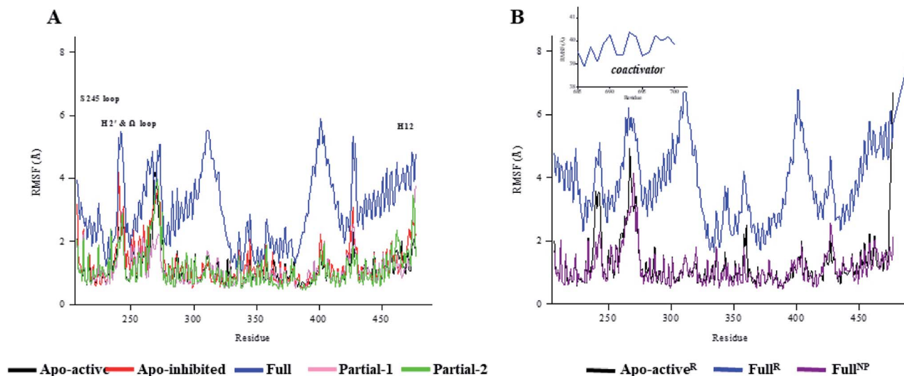
Fig. 3 The root-mean-square fluctuations (RMSF) per residue of various PPAR \gamma -LBD structures over (A) 100 ns and (B) 600 ns MD trajectories. The values of Full R were averaged based on three independent 600 ns MD trajectories. H2' & \Omega loop (residues 250–266 and residues 263–278), S245 loop (residues 237–253) and H12 (residues 465–477).
