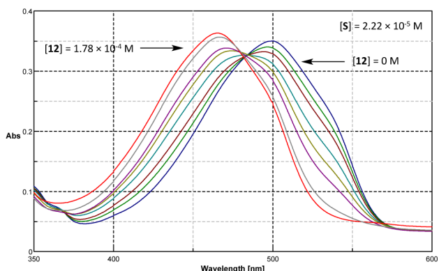
Figure 1. Response in the UV–vis spectrum of S upon increasing amounts of 12 . [S] = 2.22 \times 10^{-5} M in \text{CH}_2\text{Cl}_2 , [12] = 0 to 1.78 \times 10^{-4} M.
