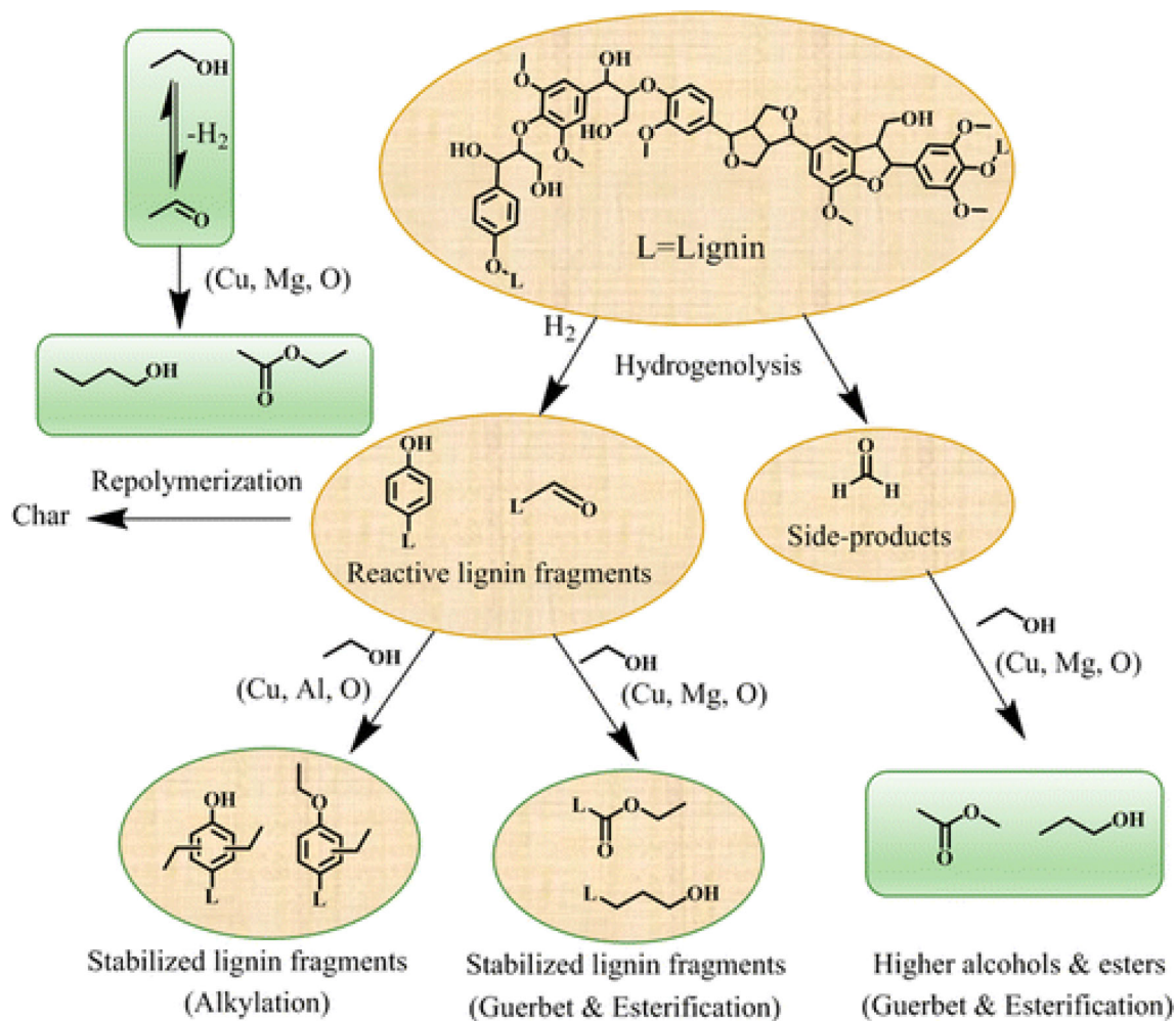
Fig. 5 Proposed reaction scheme for lignin depolymerization in ethanol over a Cu, Mg, Al catalyst. Reproduced from Ref. [40] with permission. Copyright © 2015 American Chemical Society
