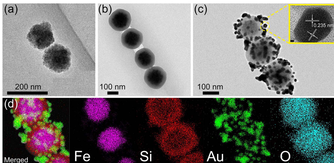
Fig. 3 (a)–(c) The TEM images of \text{Fe}_3\text{O}_4 MNPs, \text{Fe}_3\text{O}_4@SiO_2 MNPs, and Au-loaded \text{Fe}_3\text{O}_4@SiO_2 MNPs, respectively. The inset in (c) shows the high-resolution TEM (HRTEM) image of Au NPs. (d) The EDX mapping images of elements Fe (pink), Si (red), Au (green), and O (cyan) in AuMF.
