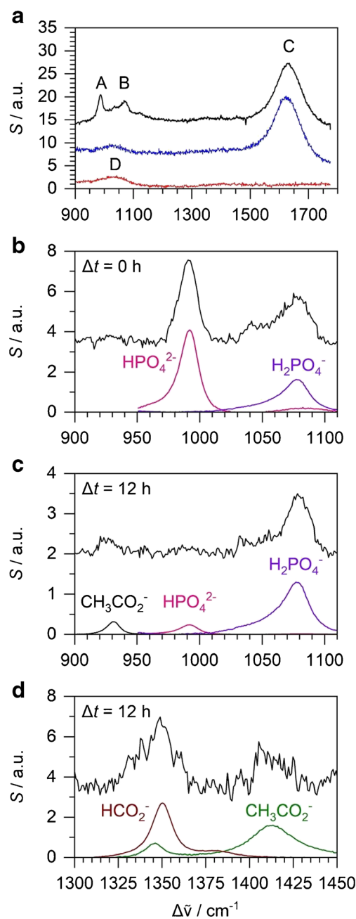
Fig. 3 Experimental Raman spectra. a Fresh M9 medium (upper trace, black), water (middle trace, blue), and empty glass tube (lower trace, red). b Bacterial suspension at the start of anaerobic fermentation with peaks due to 47 mM HPO 4 2- and 22 mM H 2 PO 4 - . c After 12 h of anaerobic fermentation with peaks due to 3 mM HPO 4 2- , 66 mM H 2 PO 4 - , and 20 mM acetate. d After 12 h of anaerobic fermentation with peaks due to 20 mM acetate and 15 mM formate
