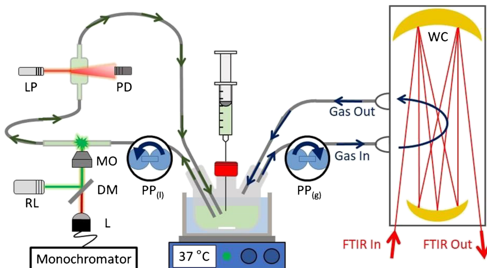
Fig. 2 Scheme of the experimental setup for spectroscopic analysis of bacterial fermentation. DM, dichroic mirror; L, lens; LP, laser pointer; MO, microscope objective; PD, photodiode; PP (g) , gas-phase peristaltic pump; PP (l) , liquid-phase peristaltic pump; RL, Raman laser; WC, White cell
