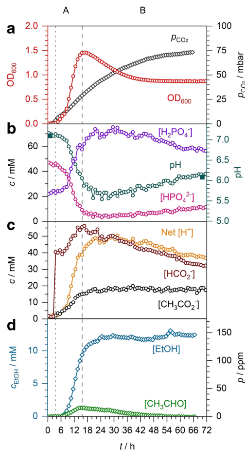
Fig. 7 E. coli anaerobic fermentation in M9 medium with 40 mM potassium formate added at 3 h as shown by a dotted line. Phases A and B denote formate accumulation and decline, respectively. a OD of the bacterial culture and partial pressure of CO_2 . b Concentrations of the phosphate buffer components with in situ, spectroscopic pH (open circles) and externally measured pH (solid squares). c Concentrations of acetate, formate, and net acid produced as quantified by Raman spectroscopy. d Partial pressures of ethanol and acetaldehyde determined by FTIR spectroscopy with calculated dissolved ethanol concentrations
