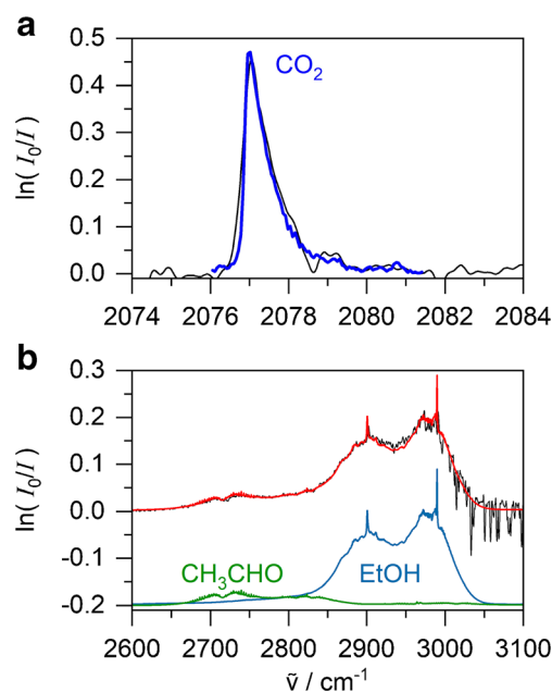
Fig. 5 FTIR spectrum taken after 12 h of E. coli with fitted PNNL model spectra. Panel a : experimental \text{CO}_2 peak corresponding to 21 mbar shown in black with fitted \text{CO}_2 model spectrum in blue. Panel b : overlapping experimental bands of acetaldehyde and ethanol corresponding to 18 and 105 ppm, respectively, shown in black. Acetaldehyde and ethanol model spectra are shown in green and blue, respectively, with the sum of both models shown in red
