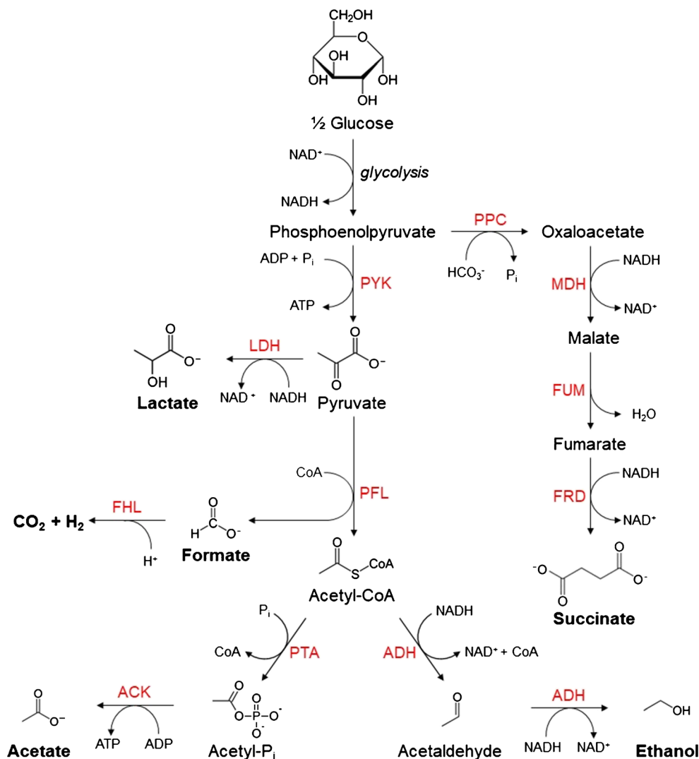
Fig. 1 E. coli mixed acid fermentation pathways with glucose as a carbon source. End products are shown in boldface. The enzymes responsible for each step are indicated in red: ACK, acetate kinase; ADH, alcohol dehydrogenase; FHL, formate hydrogenlyase; FRD, fumarate reductase; LDH, lactate dehydrogenase; MDH, malate dehydrogenase; PFL, pyruvate formate lyase; PPC, phosphoenolpyruvate carboxylase; PTA, phosphotransacetylase; PYK, pyruvate kinase
