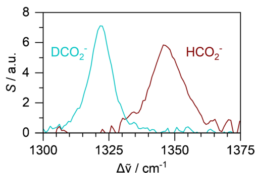
Fig. 4 Raman spectra of 40 mM deuterated (blue) and unlabelled (red) formate solutions
