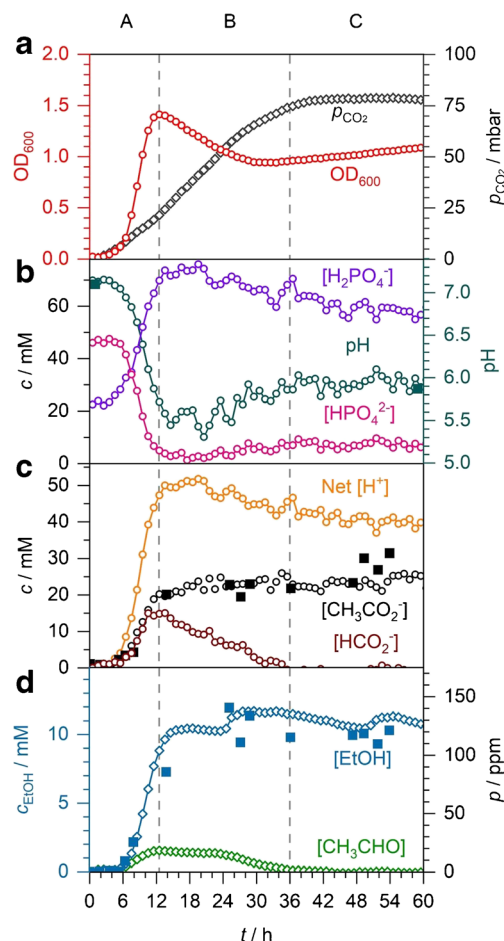
Fig. 6 E. coli anaerobic fermentation in M9 medium. A to C denote three distinct phases: formate accumulation, decline, and depletion, respectively. a OD of the bacterial culture and partial pressure of \text{CO}_2 . b Concentrations of the phosphate buffer components with in situ, spectroscopic pH (open circles) and externally measured pH (solid squares). c Concentrations of acetate, formate, and net acid produced. Acetate quantification by Raman (open circles) and GC (solid squares) is compared. d Partial pressures of ethanol and acetaldehyde. Ethanol concentrations by FTIR (open diamonds) and GC (solid squares) are compared
