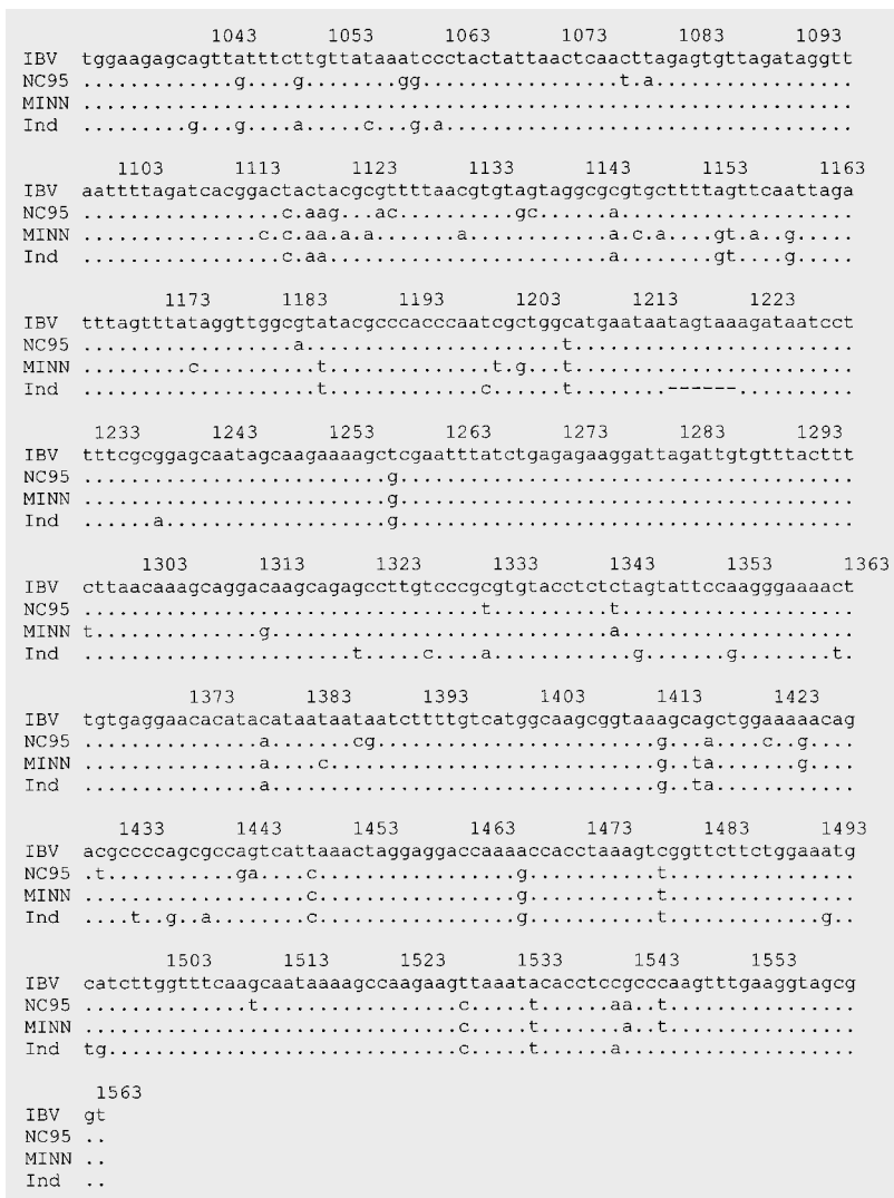
Fig. 2. Comparison of MN gene nucleotide sequence of infectious bronchitis virus (IBV) Beaudette strain [20] and TCV strains NC95, Minnesota, and Indiana. Nucleotide sequence differences are shown for TCV strains. The positions where nucleotide bases are missing are indicated as (-) and similar nucleotides as (.)
