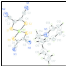
Fig. 1. The molecular structures of the ionic components of (I), showing the atom-numbering scheme and displacement ellipsoids at the 30% probability level.
