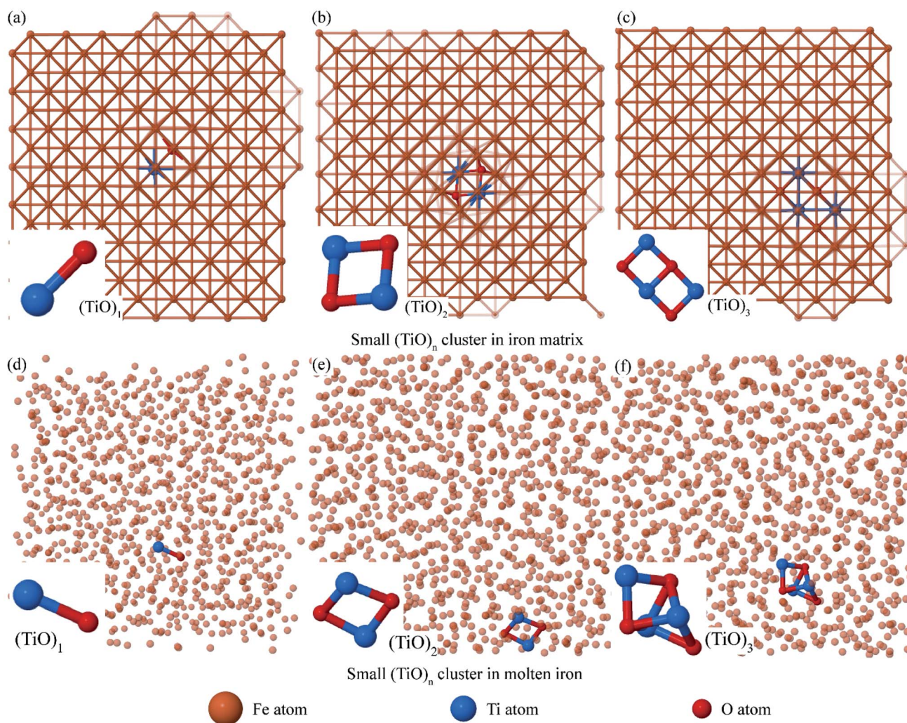
Fig. 2 Small (TiO) n clusters were optimized in an 8 × 8 × 8 iron supercell. (a)–(c) The (TiO) n cluster structure was established at 0 K. (d)–(f) (TiO) n cluster structure was optimized at T_s = 2122 K.
