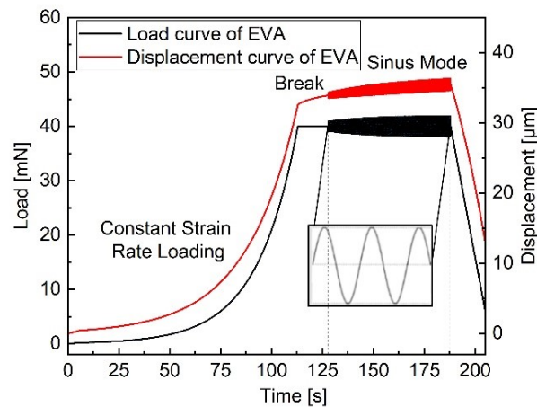
Figure 6. Dynamic load-displacement-time curves on the EVA surface obtained using a frequency sweep during the hold.
