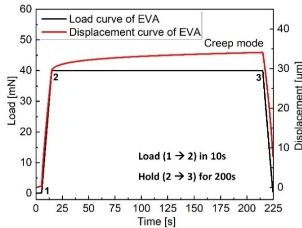
Figure 3. Creep load-displacement-time curves on the EVA surface obtained using a maximum load 40 mN, duration of creep 200 s.
