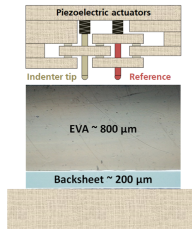
Figure 2. illustration of the Ultra Nanoindentation Head Assembly applied to the multilayer EVA-BS film.
