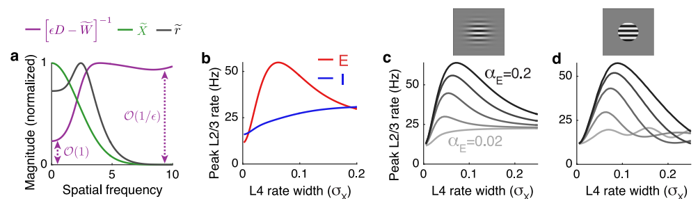
Fig 6. Spatial filtering of external input and the dependence of suppression on outgoing synaptic projection width. a The magnitude of the spatial filter, [\epsilon D - \tilde{\mathbf{W}}(n)]^{-1} , imposed by recurrent connections (purple), the external input \tilde{\mathbf{X}}(n) , (green) and the resulting firing rate profile \tilde{\mathbf{r}}(n) , (black) as a function of the spatial frequency, \|\mathbf{n}\| = \sqrt{m^2 + n^2} , from the simulation in Fig 5j–5o. Magnitude is measured by the Frobenius norm for [\epsilon D - \tilde{\mathbf{W}}(n)]^{-1} . Curves normalized by their peaks. b Firing rates of excitatory (red) and inhibitory (blue) neurons with receptive fields at the center of a grating stimulus plotted as the width of the stimulus increases (represented by increasing \sigma_X ) using parameters from Fig 5j–5o. c Same as b, but the excitatory rate is plotted for different widths of the excitatory synaptic projection width, \alpha_E . d Same as c, but firing rates in L4 are shaped like a disc with radius \sigma_X instead of a Gaussian with width parameter \sigma_X .
