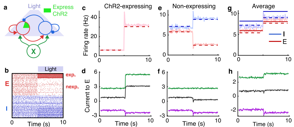
Fig 2. Imbalanced amplification and suppression under partial optogenetic stimulation. Same as Fig. 2a–d except the inward current was only provided to 20% of the excitatory neurons, modeling ChR2-expressing pyramidal cells. a) Schematic. A population of recurrently connected excitatory (red) and inhibitory (blue) spiking neuron models receive synaptic input from an external population ( X ; green) of Poisson-spiking neurons. Optogenetic stimulation of excitatory neurons was modeled by an extra inward current to 20% of the excitatory population at 5s. b) Spike rasters from 10 randomly selected ChR2-expressing and 40 non-expressing excitatory (red) neurons and 50 inhibitory (blue) neurons from the recurrent network. c) Average firing rate of ChR2-expressing excitatory neurons from simulations (light solid) and from the corrected approximation (Eq (4); dashed). d) Mean synaptic currents to 200 randomly selected ChR2-expressing excitatory neurons from external inputs ( X ; green), from the local population ( E + I ; purple) and the total synaptic current (black). e) Same as c, but for non-expressing excitatory neurons (red) and inhibitory neurons (blue). f) Same as d, but for non-expressing excitatory postsynaptic neurons. g) Same as c and d, but averaged over all excitatory neurons (expressing and non-expressing). Currents are measured in units of the neurons’ rheobase (rheobase/ C_m = 10.5 V/s). Firing rates predicted by Eq (3) are not shown in c and e because Eq (3) is not applicable to those cases.
