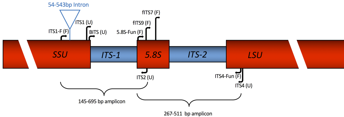
FIG 1 Fungal nuclear ribosomal ITS primer map. Blocks in red are the SSU (18S or small subunit nuclear rRNA gene), 5.8S (also a structural RNA gene), and LSU (28S or large subunit nuclear rRNA gene). The blue triangle above the SSU gene indicates the type I self-splicing intron insertion site. The two transcribed but nonstructural spacer regions, ITS-1 and ITS-2, are shown in blue blocks. Primer names and relative positions are given. In parentheses, F indicates primers that were designed to select against nonfungal taxa; U indicates primers that were designed as universal eukaryote primers. While designed to be selective for Fungi, ITS1-F has the potential to amplify a range of protist lineages (see Fig. S2 in the supplemental material). Primers fITS7 and fITS9 were designed to be fungal selective but have the potential to amplify diverse plants, according to our in silico analyses and empirical reports of the authors (27). Primers fITS9 and ITS2 are unlikely to amplify some important fungal lineages, according to our in silico analyses (see Fig. S3 in the supplemental material). At the bottom are estimates of the range of amplicon lengths, including taxa with and without the 3' SSU intron, based on the ITS-LSU OTU representative sequences from reference 4. Gene sizes and primer positions are not to scale.
