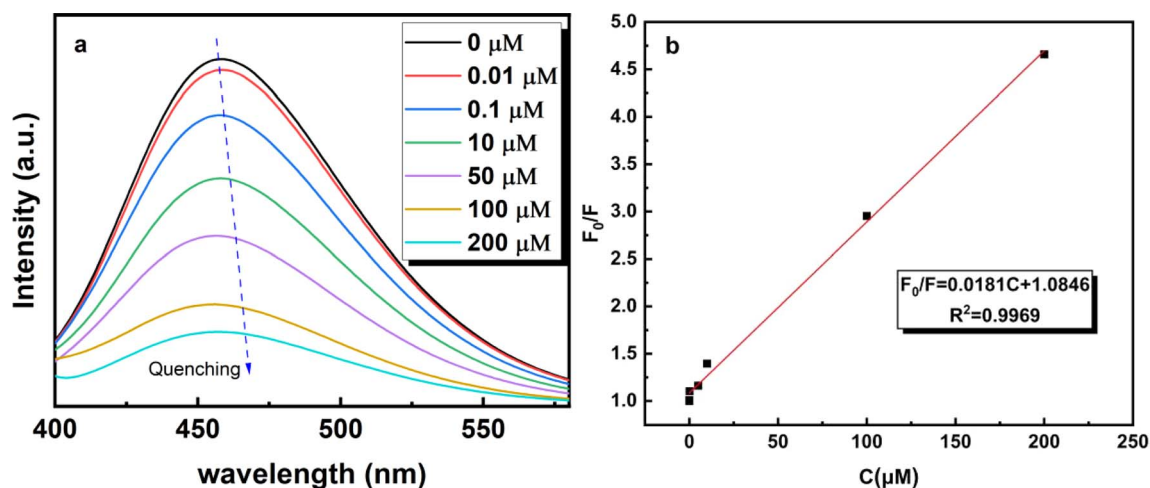
Fig. 9 (a) Fluorescence emission spectra of b-CDs in Fe^{3+} solutions with varying concentrations from 0.01 to 200 \mu M. (b) Fitting curve of F_0/F as a function of Fe^{3+} ion concentration for b-CDs.
