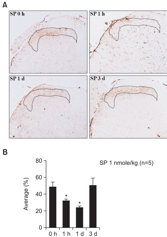
Fig. 2. The expression of phospho-ERK in the spinal cord is decreased by the intravenous administration of SP: (A) Immunohistochemical analysis of phospho-ERK in the lamina I-II at the L4-L5 level of the spinal cord, as indicated by the dotted line, showed reduced immunoreactivity following the i.v. administration of SP intravenously in the neuropathic pain model. The expression was decreased at 1 h after injection, remained low for 1 d post-injection, and increased again 3 d post-injection. Scale bar: 50 \mu m. (B) The statistical summary of the immunohistochemically positive stained area from five independent results of immunocytochemistry ( *p < 0.05 ). Mean percentages (%) of phospho-ERK-immunoreactive (IR) neurons relative to the total number of neurons at the L4-L5 level of the spinal cord. Data are presented as means \pm SEM.
