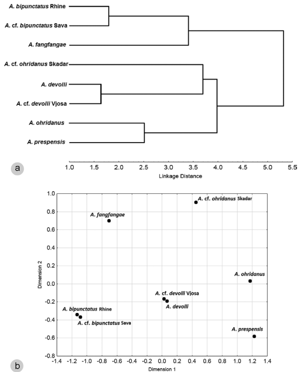
Figure 2. a Cluster analysis b multidimensional scaling results for Alburnoides samples of North, Black, and Adriatic basins from Rhine southwards to Vjosa in Albania based on data for counts and coded qualitative characters as in Table 3. Adriatic samples of Alburnoides prespensis complex named as presumed species.
