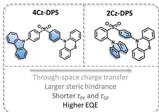
Fig. 1 Molecular structures of 4Cz-DPS and 2Cz-DPS .
