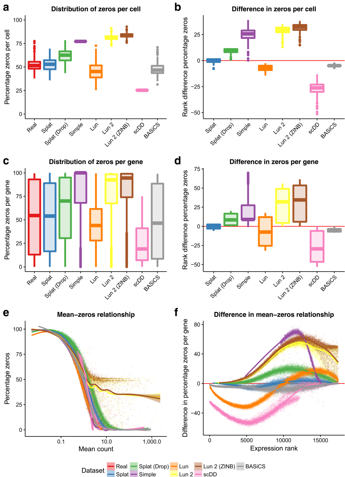
Fig. 3 Comparison of zeros in simulations based on the Tung dataset. The top row shows boxplots of the distribution of zeros per cell ( a ) and the difference from the real data ( b ). The distribution ( c ) and difference ( d ) in zeros per gene are shown in the middle row . The bottom row shows scatter plots of the relationship between the mean expression of a gene (including cells with zero counts) and the percentage of zeros as both the raw observations ( e ) and ranked differences from the real data ( f )
