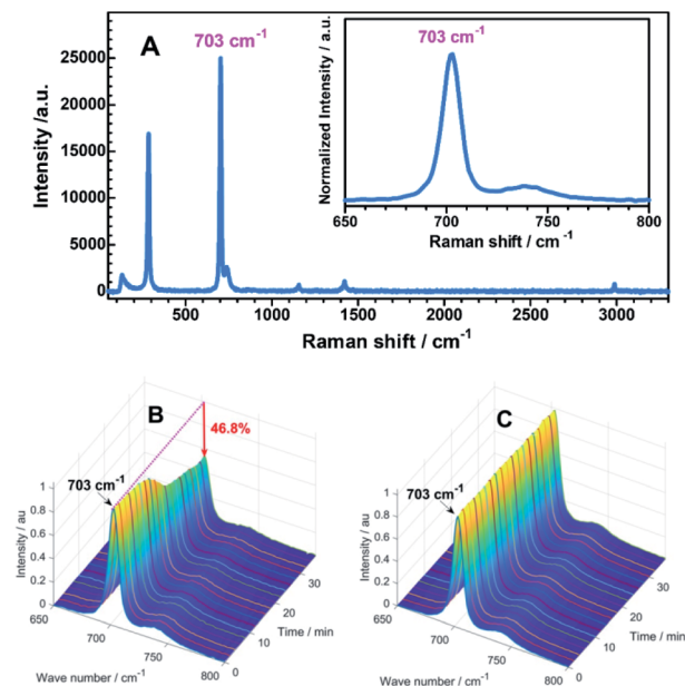
Fig. 4 Typical Raman spectrum of pure DCM (A); variation of the Raman peak (703 cm -1 ) of DCM with UV-exposure time in the presence (B) and absence (C) of OAm-PNCs.
