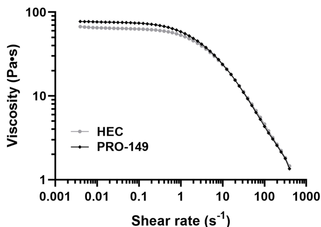
Figure 1 Shear rate ( s^{-1} ) versus average viscosity (Pascal second) for test OVD (PRO-149) compared to control OVD (HEC) in logarithmic scale. Data from 3 batches.
