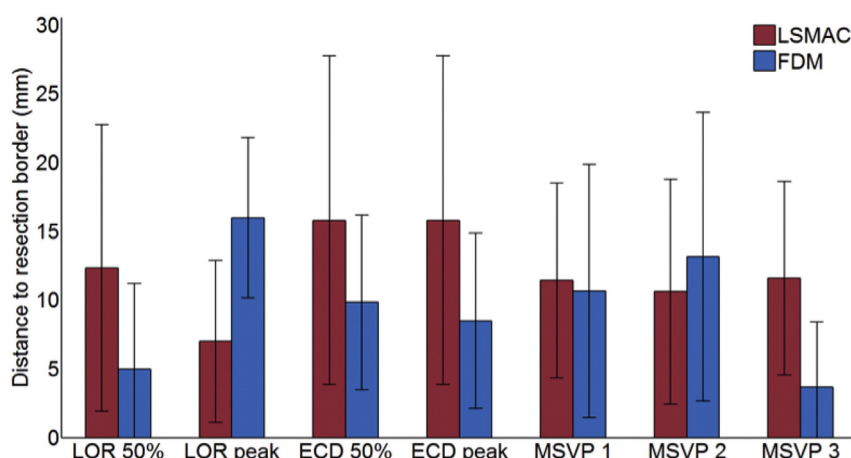
Fig. 6. Comparison of the distances to the border of the resection for the LORETA, ECD and MSVP approaches using the LSMAC and FDM forward models respectively. LOR 50%: LORETA at 50% of the peak, LOR peak: LORETA at the peak, MSVP 1: MSVP (−50 ms to 50% peak), MSVP 2: MSVP (−50 ms to peak), MSVP 3: MSVP (−50 ms to 230 ms). The error bars denote the standard deviation over the 6 patients.
