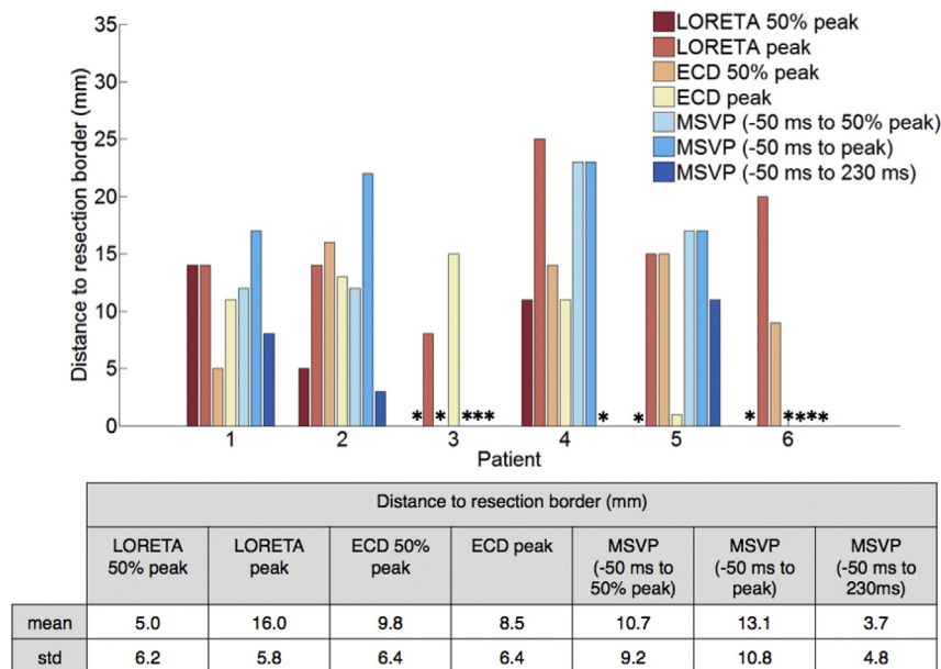
Fig. 5. The distance to the resection border, d_r (in mm) for each of the patients (P1 to P6) and for the different methods. In the table below, the means and standard deviations of each method are given. The stars denote the situations in which the activity was correctly estimated inside the resected area.
