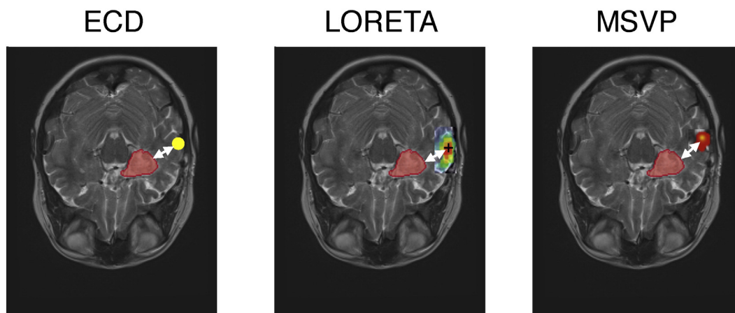
Fig. 3. Illustration of the distance to the border of the resection for each of the considered approaches. For the LORETA and MSVP approaches, the maximum estimated intensity of the dipole in the distributed source model is used to calculate the distance.
