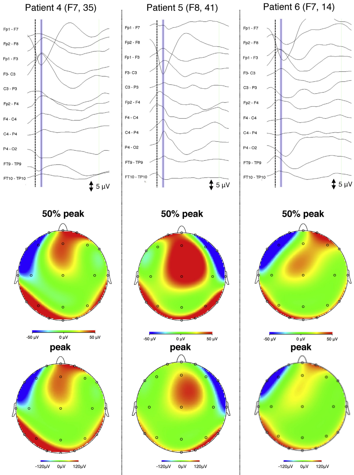
Fig. 2. The averaged spikes and topographies corresponding with the spike peak and at 50% of the spike peak for the 27 channels recordings in patients 4 to 6. The vertical dashed lines correspond with 50% of the spike peak during the rising phase of the peak. The channel to select the peak of the spike and the number of spikes that were averaged are given for each patient.
