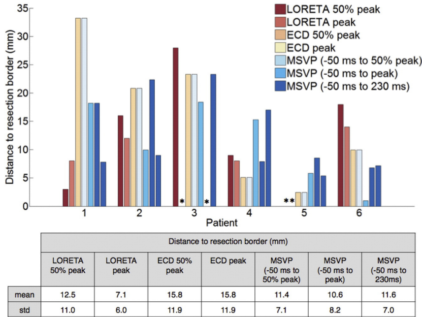
Fig. 4. The distance to the resection border, d_r (in mm) for each of the patients (P1 to P6) and for the different inversion methods. In the table below, the means and standard deviations of each method are given. The stars denote the situations in which the activity was correctly estimated inside the resected area.
