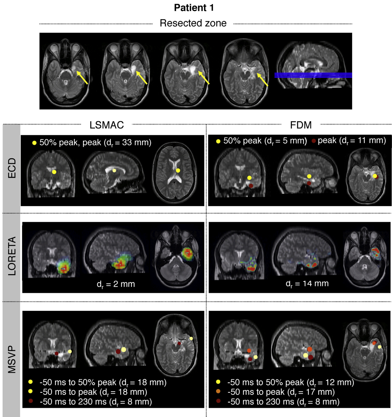
Fig. 7. First row: illustration of the resected zone of patient 1 in different horizontal slices. The results below are depicted by the rows corresponding with the inversion approaches and the columns representing the forward models. For the LORETA approaches the results are shown corresponding with the activity at 50% of the peak of the spike.
