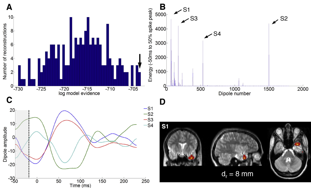
Fig. 8. Panel A: histogram of the free energy values corresponding with the with the MSVP inversions. Panel B: energy of the dipole intensities based on the MSVP solution. The dipoles with the maximum energy are depicted by S1, S2, S3 and S4. Panel C: the time courses of S1, S2, S3 and S4. Panel D: the location of volumetric region shown on top of the resected zone in 3 orthogonal slices corresponding with S1.
