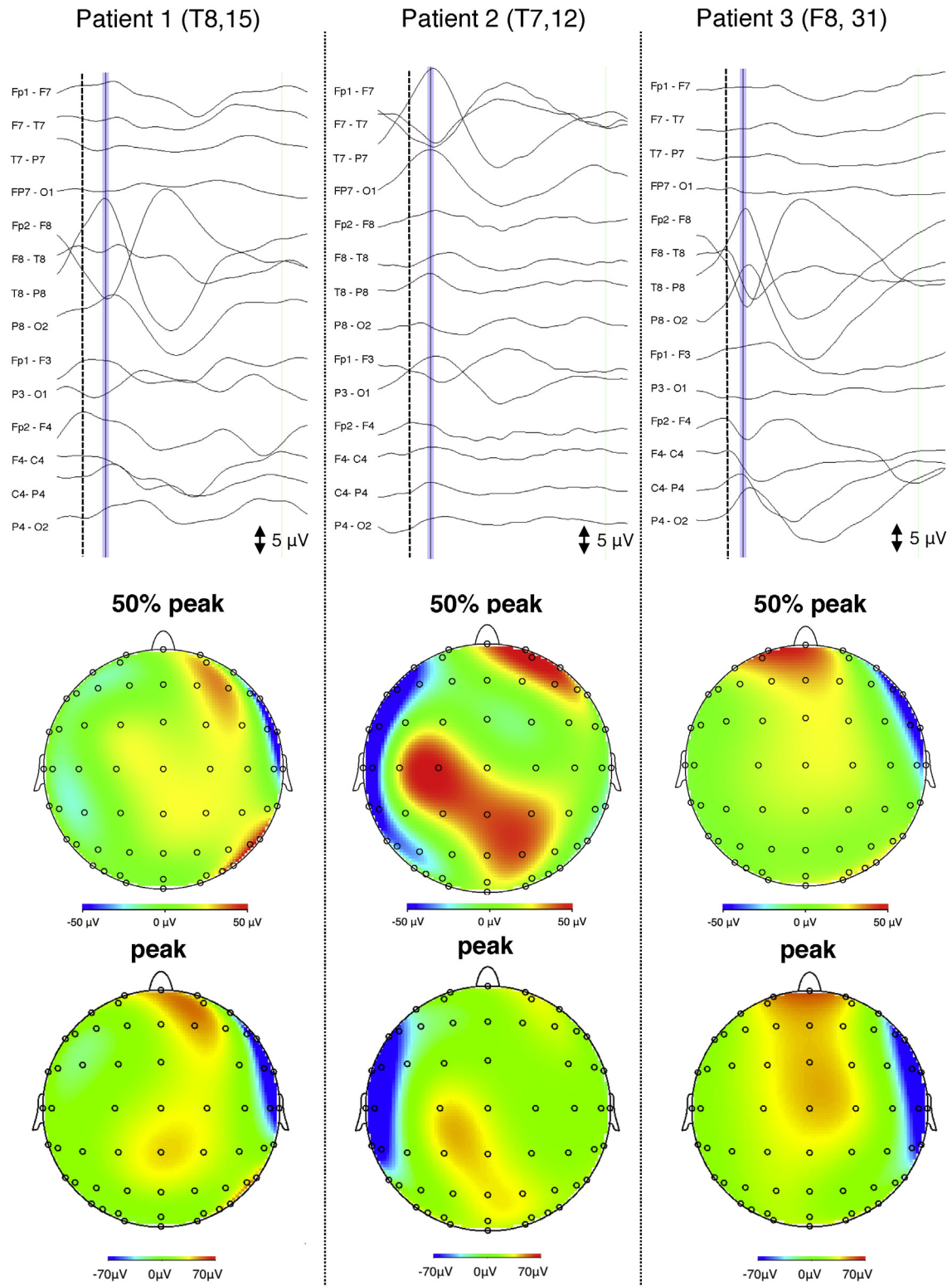
Fig. 1. The averaged spikes and topographies corresponding with the spike peak and at 50% of the spike peak for the 64 channels recordings in patients 1 to 3. The vertical blue lines correspond with the spike peaks. The vertical dashed lines correspond with 50% of the spike peak during the rising phase of the peak. The channel to select the peak of the spike and the number of spikes that were averaged are given for each patient. (For interpretation of the references to color in this figure legend, the reader is referred to the web version of this article.)
