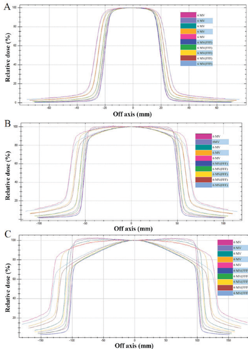
Figure 1. The off axis curve of 6X and FFF in different depths. (A) The off axis response to dose distribution in the control group was similar in the 6X and FFF model. (B and C) The off axis responses in the experimental groups were significantly larger in the 6X model compared with the FFF model. FFF, flattening filter-free.
