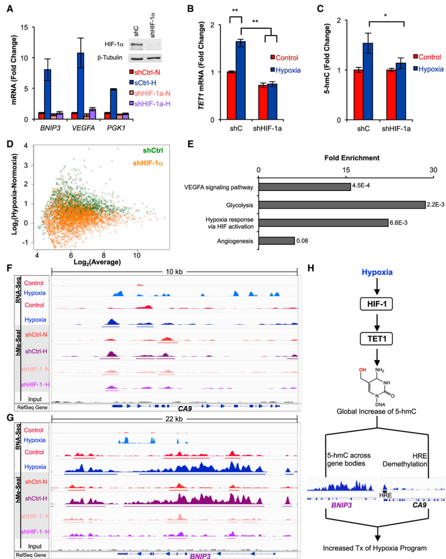
Figure 4. HIF-1 Regulates TET1 and Is Necessary for Genome-wide and Locus-Specific 5-hmC Gains in SK-N-BE(2) Cells
