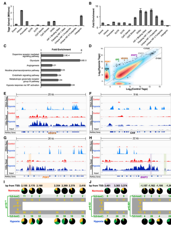
Figure 2. 5-hmC Gains Occur at Hypoxia Regulated Regions in SK-N-BE(2) Cells (A and B) Absolute 5-hmC gains (A) and enrichment for 5-hmC gains (B) were calculated at genomic elements. Regions flanking HIF binding sites are regions \pm 1 kb from the ChIP-seq peak. Footprints include the ChIP-seq peak and flanking region (Schödel et al., 2011). Data represent means \pm SD for two biological replicates. (C) PANTHER pathway analysis of genes with regions gaining at least 3-fold 5-hmC. p values are Bonferroni corrected results of binomial tests (Mi et al., 2013). (D) Regions gaining the most 5-hmC map to the HIF-1 target genes CA9 , PGK1 , GPI , VEGFA , BNIP3 , and ENO1 . Plotted points represent combined data from two experiments. (E–H) RNA-seq and hMe-Seal sequencing data are plotted in the Integrated Genomics Viewer (IGV) genome browser at VEGFA , CA9 , PGK1 , and BNIP3 genes. RefSeq gene tracks represent the position of known genes in the hg19 build of the human genome. Arrows represent the direction of transcription. (I and J) TAB-seq data for the corresponding shaded regions of PGK1 (G) and BNIP3 (H). For each CpG, black, green, and gold represent the percentage of 5-mC, 5-hmC, and unmodified cytosine, respectively. Results represent pooled data over three independent experiments. p values calculated by chi-square tests. See also Figure S2 and Table S2.
