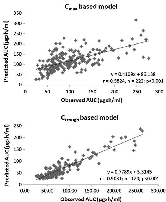
Fig. 3 Correlation of the observed vs. predicted values for either the linezolid C_{\text{max}} model or the linezolid C_{\text{trough}} model. AUC area under the plasma concentration–time curve, C_{\text{max}} maximum plasma drug concentration, C_{\text{trough}} trough plasma concentration
